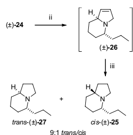
Scheme 9: i) \text{CH}_3\text{OH} , Zn, conc. \text{HCl(aq)} ii) \text{H}_2 (40 psi), Pd/C, EtOH, 2 M HCl
