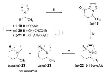
Scheme 7: Reaction conditions: i) DIBAL-H, \text{CH}_2\text{Cl}_2 , -78^\circ\text{C} , 1 h then triethylphosphonoacetate, NaH, THF, -78^\circ\text{C} - rt ii) \text{H}_2 (40 psi), Pd/C, EtOH iii) \text{BBr}_3 , \text{CH}_2\text{Cl}_2 , 0^\circ\text{C} , 10 min iv) Zn, conc. HCl(aq) v) \text{H}_2 (40 psi), Pd/C, EtOH, 2 M HCl
