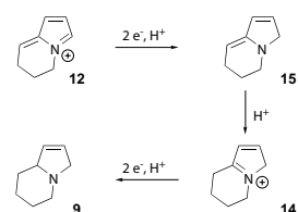
Scheme 5: Alternative reduction pathway
