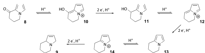
Scheme 4: Potential mechanism for \alpha -ketopyrrole reduction
