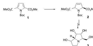
Scheme 1: Donohoe's approach to ( \pm )-1-epi-australine utilising a modified Birch reduction
