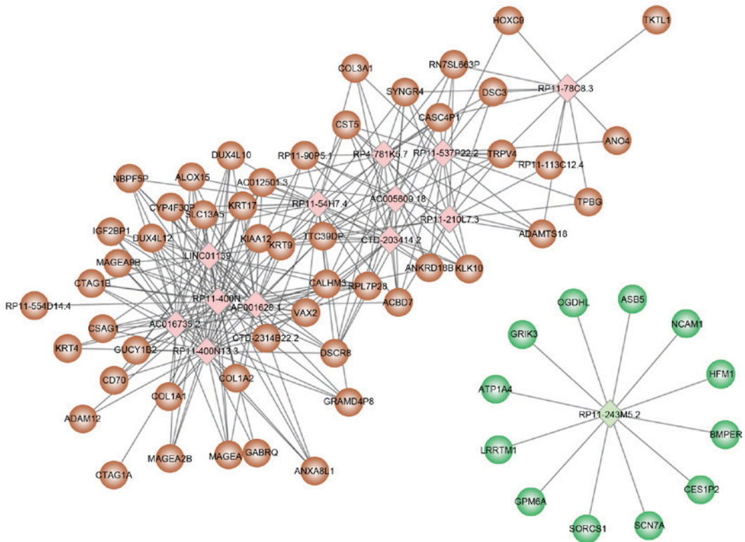
Figure 2. Regulatory network constructed with 13 lncRNAs and their target genes. Brown circles indicate upregulated target genes and green circles represent downregulated target genes. Pink rhombus, upregulated lncRNA; green rhombus, downregulated lncRNA. lncRNA, long noncoding RNA.
