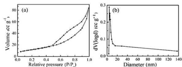
Fig. 4 \text{N}_2 adsorption and desorption isotherms of the samples obtained at 300\text{ }^\circ\text{C} . (a) Specific surface area (BET) (b) pore-size distribution (BJH).
