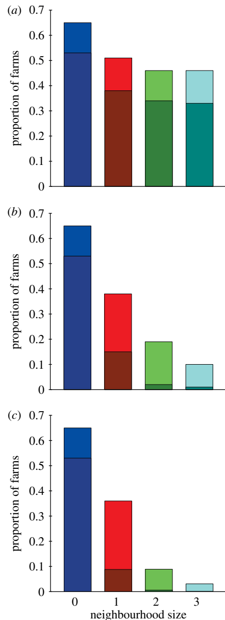
Figure 4. Proportion of farms infested (whole bar) and symptomatic (darker section) in 2090 for partially resistant varieties causing (a) 80% reduction in inoculum returned to the soil relative to susceptible varieties, (b) 99% reduction and (c) 100% reduction (fully resistant). Resistant varieties are deployed in response to rhizomania symptoms within the given response neighbourhoods ( x -axes). The results shown correspond to 20 iterations.
