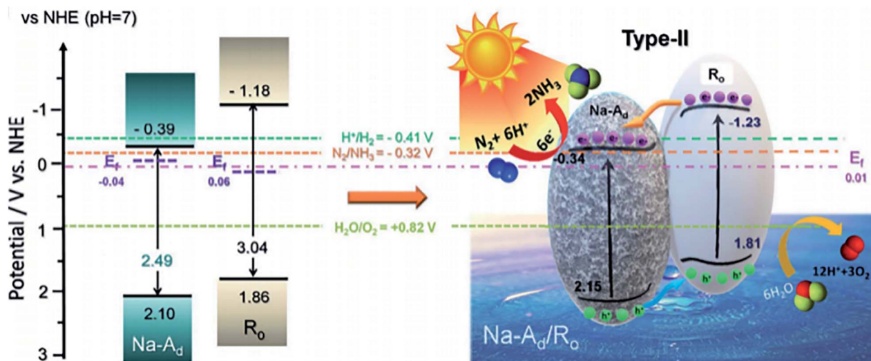
Fig. 5 Energy band structure of disordered \text{TiO}_2 (short for Na- A_d ) and ordered \text{TiO}_2 (represented by R_o ) as well as the reaction mechanism. This figure has been adapted from ref. 92 with permission from Royal Society of Chemistry, copyright 2020.
