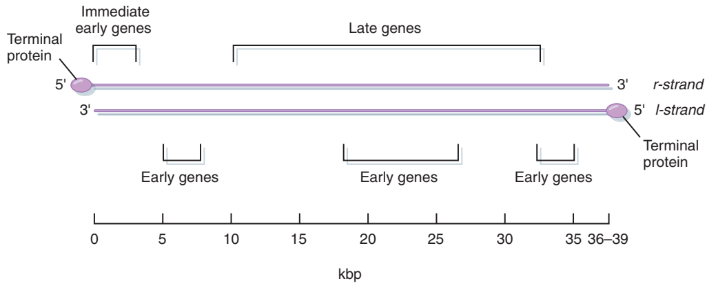
FIGURE 3.9 Adenovirus genomes. Organization of the adenovirus genome.
