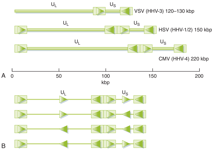
FIGURE 3.10 Herpesvirus genomes. (A) Some herpesvirus genomes consist of two covalently joined sections, U_L and U_S , each bounded by inverted repeats. (B) This organization permits the formation of four different isomeric forms of the genome.
