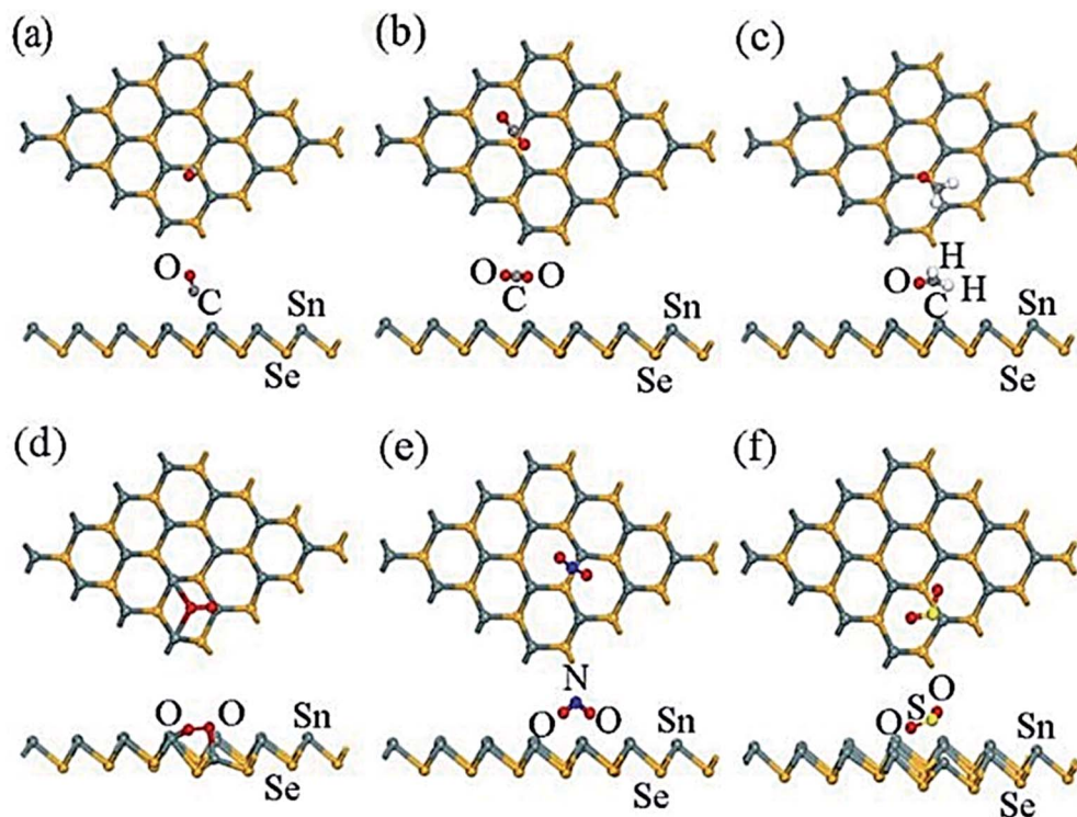
Fig. 13 The most stable sites of optimized configurations of the adsorbate molecules: (a) CO, (b) CO 2 , (c) CH 2 O, (d) O 2 , (e) NO 2 , and (f) SO 2 adsorbed on a \beta -SnSe monolayer. Most stable sites are exhibited. These figures have been adapted/reproduced 185 with permission from MDPI, copyright 2019*.
