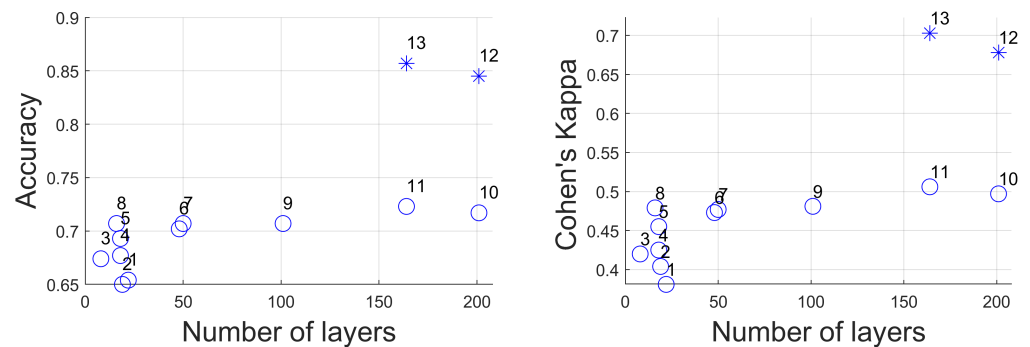
Figure 12. Illustration of the effect of the number of layers of architectures against the two metrics used in this paper Accuracy and Cohen's Kappa. Each architecture is represented by a circle, except those with augmentation that are represented by an asterisk. For visualisation purposes, numbers are added and these correspond to the order of Table 7 (1 GoogleNet, 2 VGG-19, 3 AlexNet, 4 SqueezeNet, 5 ResNet-18, 6 Inception-v3, 7 ResNet-50, 8 VGG-16, 9 ResNet-101, 10 DenseNet-201, 11 Inception-ResNet-v2, 12 ResNet-50 (augmentation), 13 Inception-ResNet-v2 (augmentation)). Notice the slight improvement provided by deeper networks and the significant improvement that corresponds to data augmentation.
