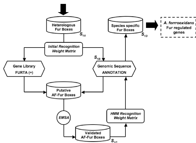
Figure 1. Pipeline for the computational and experimental steps used to identify candidate Fur-binding sites in A. ferrooxidans . Additional information and results can be found in Supplementary Data S1.
