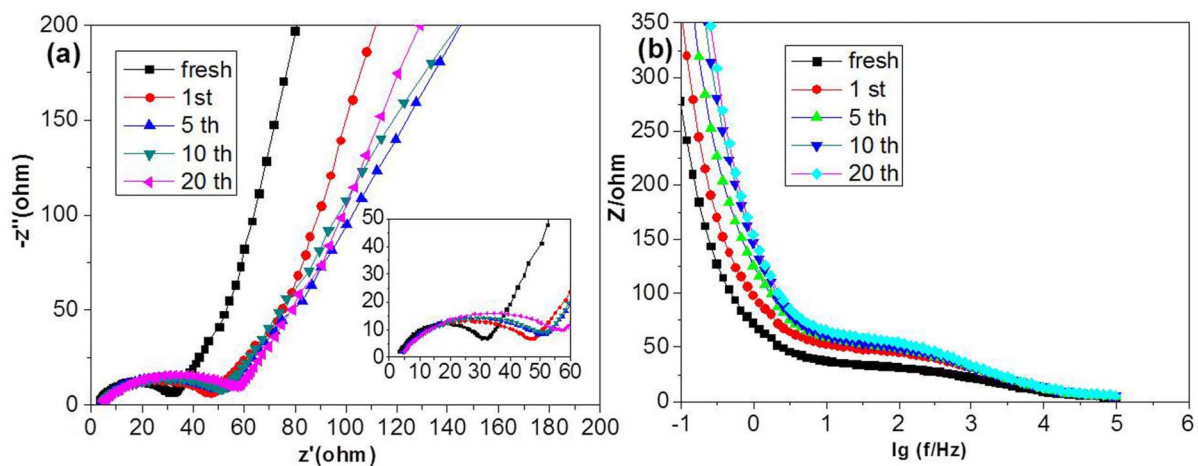
Figure 7 | Electrochemical impedance spectra and Bode plots of the \text{CoMn}_2\text{O}_4 hierarchical microspheres electrode. (a) The impedance spectra of \text{CoMn}_2\text{O}_4 electrode after different cycles of discharge and recharge at 100 \text{ mA g}^{-1} . (b) Bode plots after different cycles.
