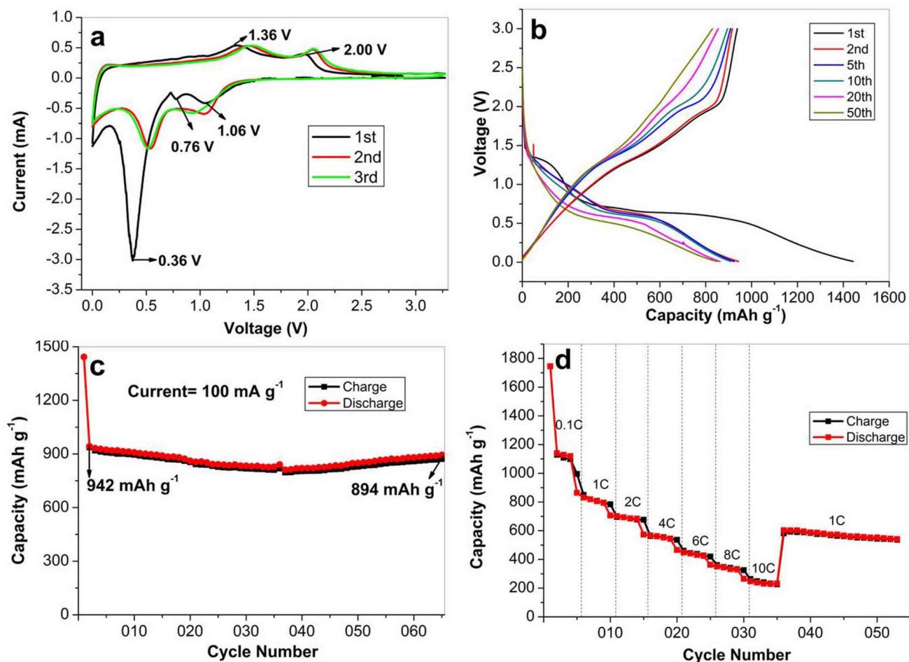
Figure 5 | Electrochemical properties of the \text{CoMn}_2\text{O}_4 hierarchical microspheres for lithium storage. (a) The first three consecutive CVs of the electrode made from \text{CoMn}_2\text{O}_4 hierarchical microspheres. (b) discharge-charge curves at a current of 100 \text{ mA g}^{-1} . (c) Cycling performance of the \text{CoMn}_2\text{O}_4 hierarchical microspheres at a current of 100 \text{ mA g}^{-1} . (d) Cycling performance of the \text{CoMn}_2\text{O}_4 hierarchical microspheres at various current rates from 0.1 C to 10 C (1 C = 900 \text{ mA g}^{-1} ). As for a half cell, the discharge process corresponds to the \text{Li}^+ insertion for \text{CoMn}_2\text{O}_4 reduction reaction, while the charge process corresponds to \text{Li}^+ extraction for \text{CoMn}_2\text{O}_4 oxidation reaction.
