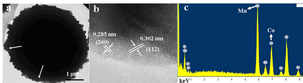
Figure 4 | Morphological and elemental analysis of \text{CoMn}_2\text{O}_4 hierarchical microspheres. (a, b) TEM and HRTEM images of \text{CoMn}_2\text{O}_4 hierarchical microspheres. (c) EDS spectrum of the \text{CoMn}_2\text{O}_4 hierarchical microspheres.
