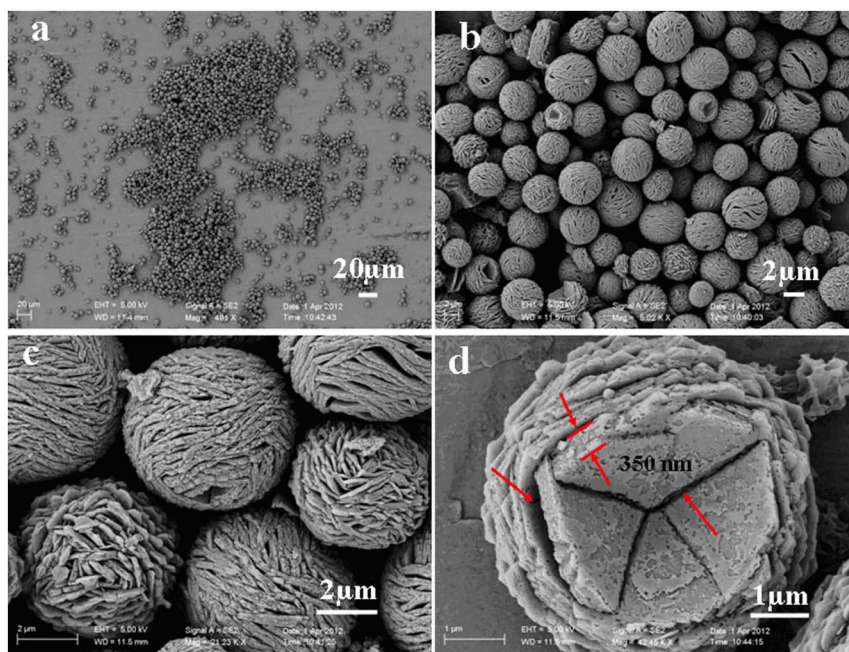
Figure 3 | Morphological and structural analysis of \text{CoMn}_2\text{O}_4 hierarchical microspheres. SEM images of the \text{CoMn}_2\text{O}_4 hierarchical microspheres at different magnifications.
