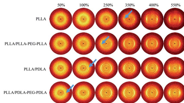
Fig. 9 WAXD patterns of PLLA and the blends with different strains at 80^\circ\text{C} . The stretching direction was vertical with a speed of 150 \mu\text{m s}^{-1} . Arrows indicate the diffraction of homocrystals.
