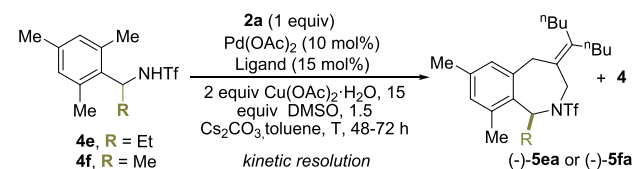
Scheme 4. Preliminary Results on a (5 + 2) Enantioselective Annulation a
