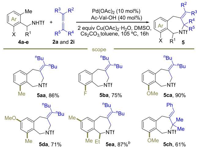
Scheme 3. Scope of the (5 + 2) Formal Cycloaddition of ortho -Methylbenzylamides and Allenes a
