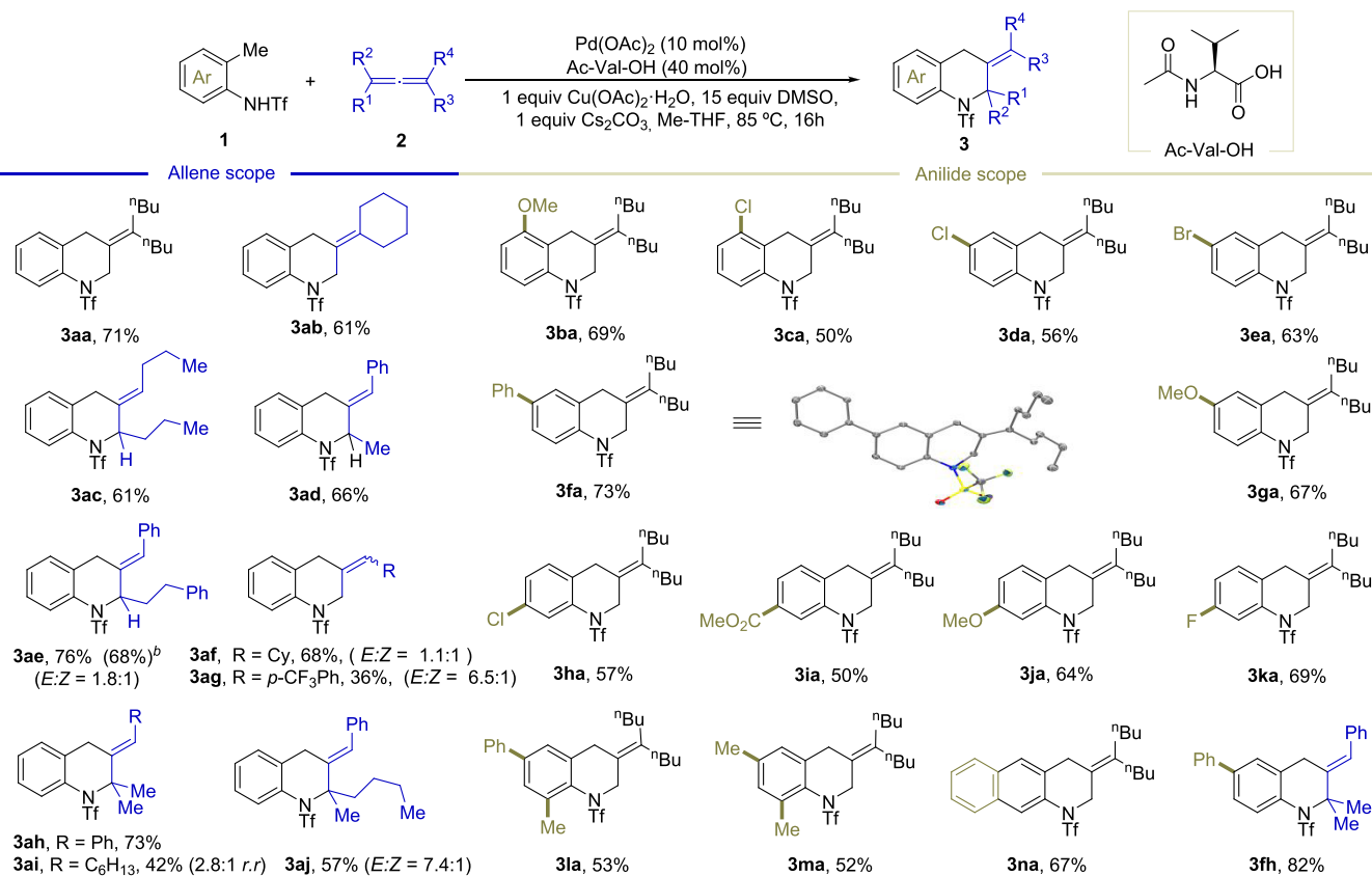
Scheme 2. Scope of the Formal (4 + 2) Cycloaddition of ortho -Anilides and Allenes a
