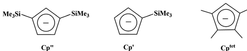
Scheme 1 Chemical structures of Cp'', Cp', and Cp tet ligands used in this study.
