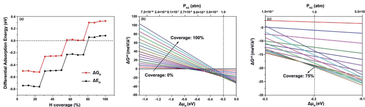
Fig. 5 (a) \Delta E_{\text{H}} and \Delta G_{\text{H}} values at various hydrogen coverages on the (100) facet; and \Delta G^{\text{ad}} at 298 K with \Delta\mu_{\text{H}} ranging from (b) -1.5 to 0.0 eV and (c) -0.3 to -0.1 eV.
