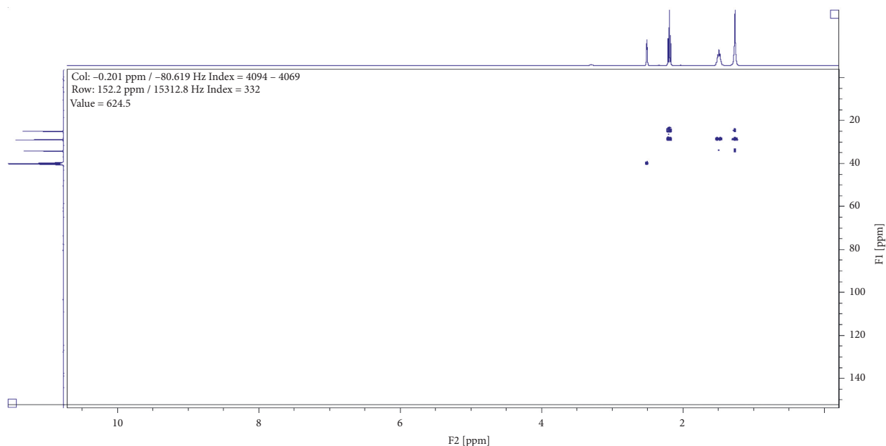
FIGURE 8: Heteronuclear multiple bond coherence profile for compound (2).
