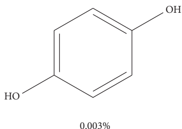
FIGURE 11: Proposed structure of compound (1): benzene-1,4-diol.
