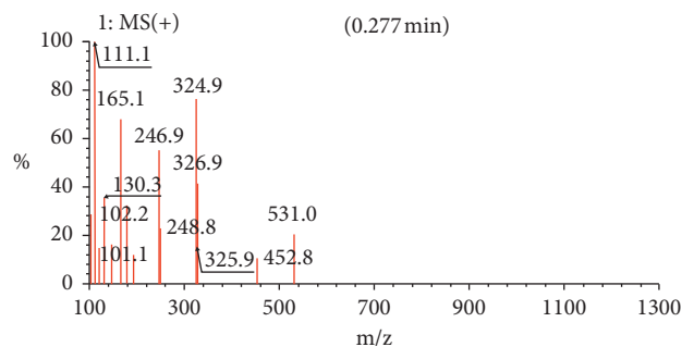
FIGURE 12: LCMS spectrum for compound (1).
