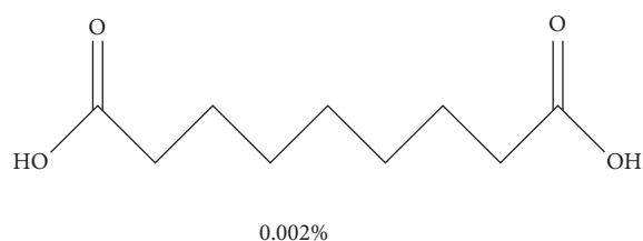
FIGURE 13: Proposed structure of compound 2: nonanedioic acid.
