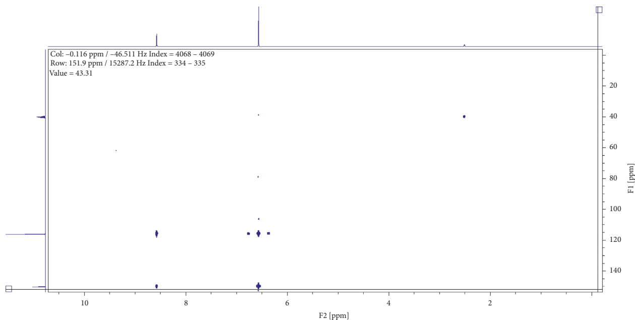
FIGURE 3: Heteronuclear multiple bond coherence profile for compound (1).
