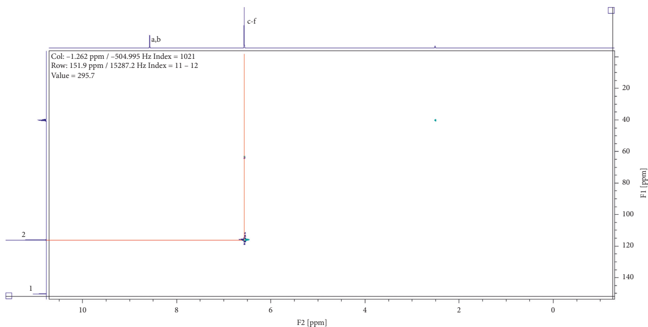
FIGURE 2: Heteronuclear single quantum coherence spectroscopy profile for compound (1).
