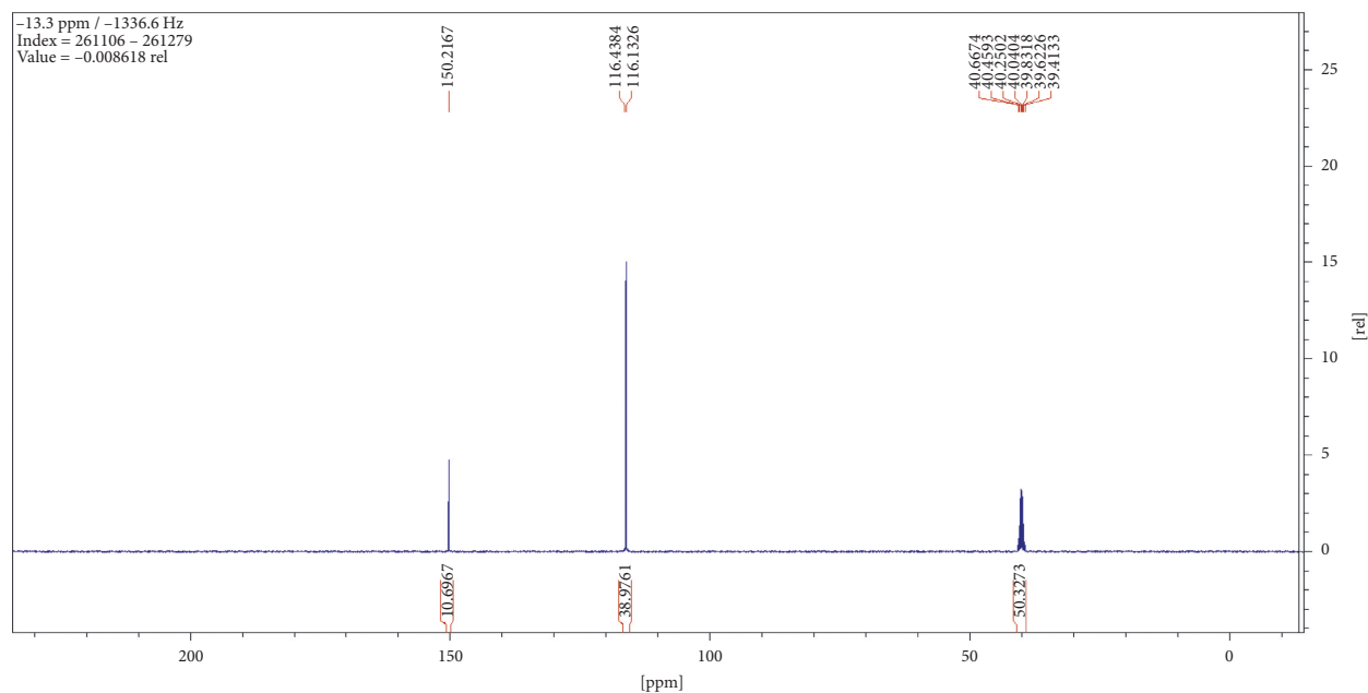
FIGURE 5: 13 C-nuclear spectroscopy profile for compound (1).
