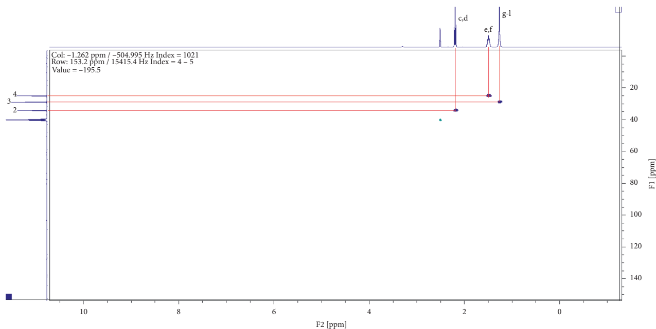
FIGURE 7: Heteronuclear single quantum coherence spectroscopy profile for compound (2).
