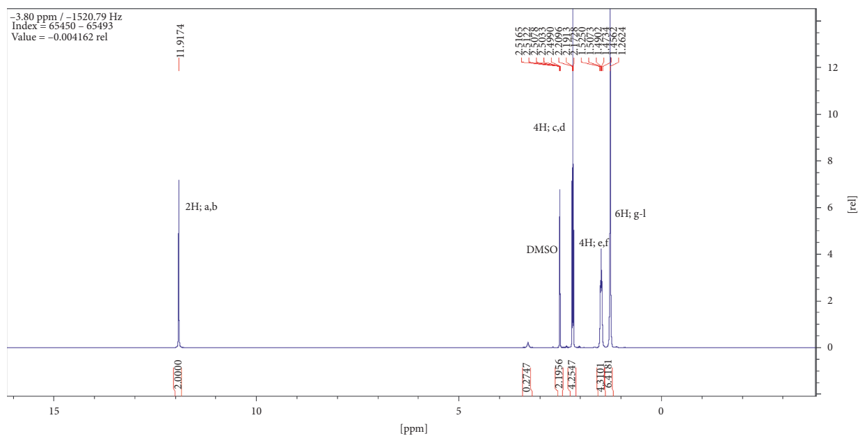
FIGURE 6: Proton nuclear magnetic resonance spectroscopy profile for compound (2).
