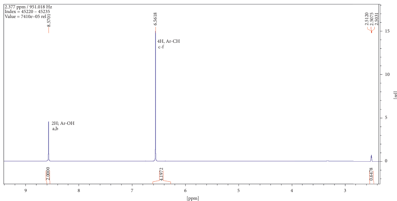
FIGURE 1: Proton nuclear magnetic resonance spectroscopy profile for compound (1).
