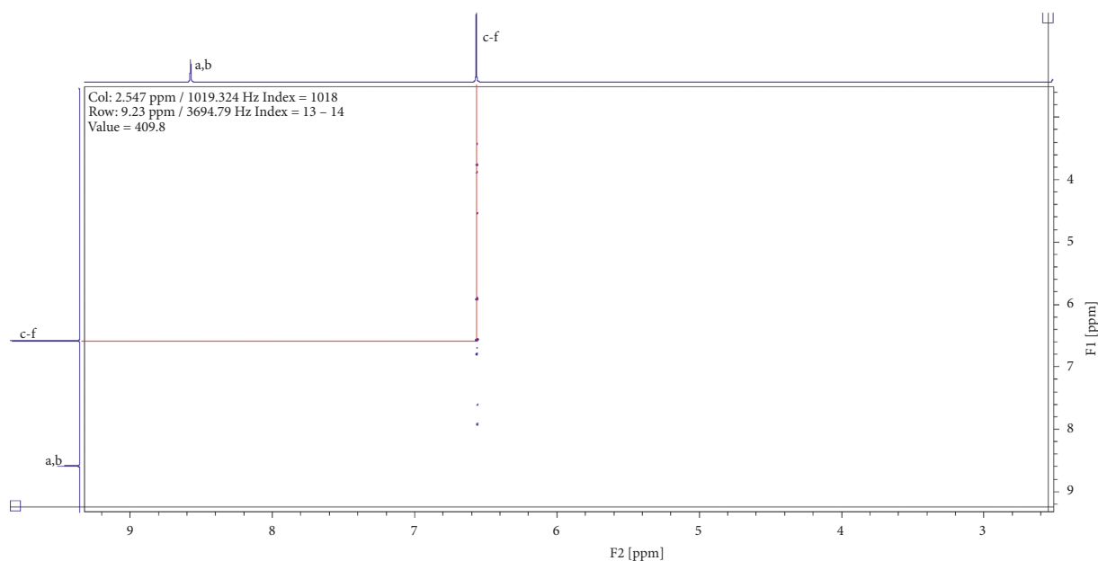
FIGURE 4: Proton-proton correlated spectroscopy profile for compound (1).
