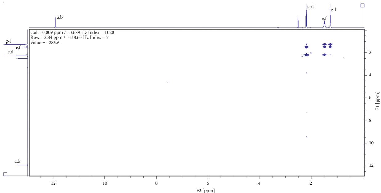
FIGURE 9: Proton-proton correlated spectroscopy profile for compound (2).
