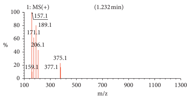
FIGURE 14: LCMS spectrum for compound (2).
