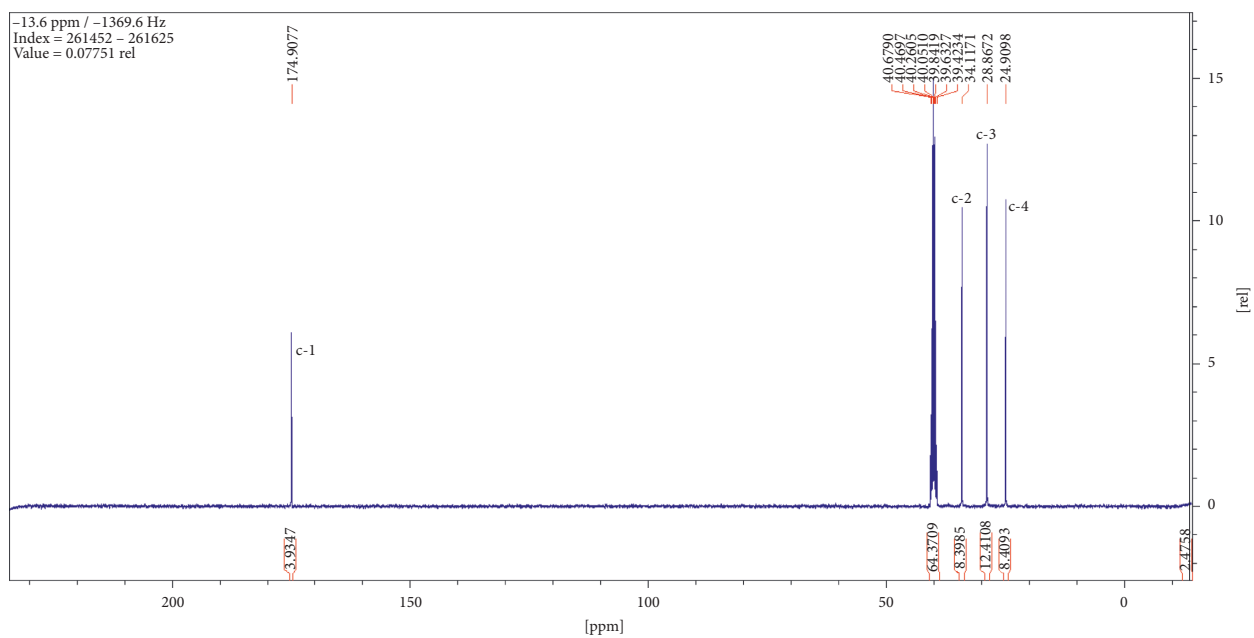
FIGURE 10: 13-carbon spectroscopy profile for compound (2).
