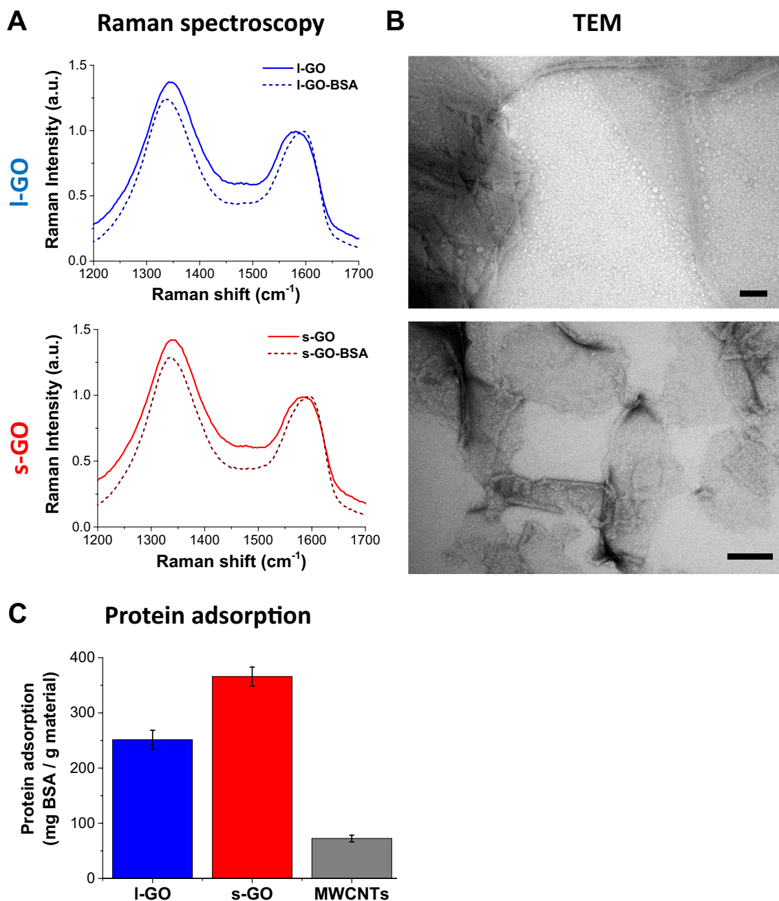
Fig. 7 Interactions of GO sheets with proteins in dispersion. a Interactions between BSA and GO sheets were probed by Raman spectroscopy, which revealed a blueshift in the G band and a reduction of I_D/I_G ratio in the presence of BSA. b TEM images illustrated the coverage of I-GO and s-GO sheets with adsorbed molecules. Scale
