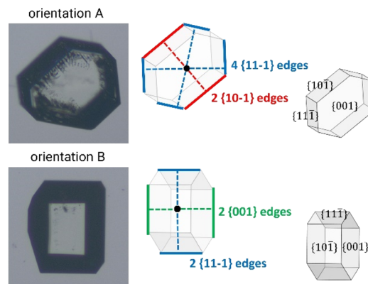
Fig. 1 The two orientations in which the crystal seeds of TFA-IX were measured. In orientation A, the distances of two edges of the \{10-1\} facets and of four edges of the \{11-1\} facets from the crystal's centroid were measured. In orientation B, the distances of two edges of the \{11-1\} facets and of two edges of the \{001\} facets from the crystal's centroid were measured.
