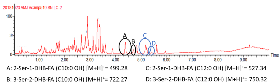
Fig. 2 LC–MS of the Vibrio campbellii CAIM 519T supernatant. Peaks A–D correlate to masses of predicted amphi-enterobactin fragments
