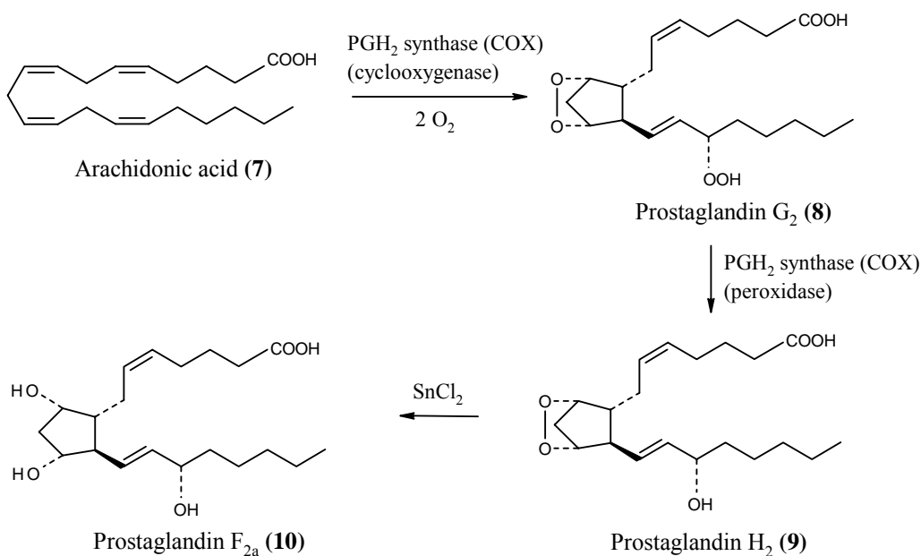
Figure 2: COX enzyme assay – conversion of arachidonic acid to prostaglandin F 2α (adapted from [28])
