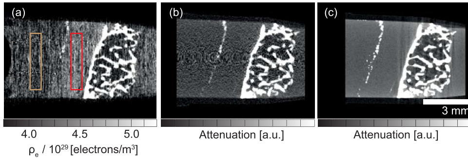
FIG. 4. Qualitative comparison of registered cross-sections of the knee joint sample obtained in phase- and absorption-contrast modes: Laboratory-based double-grating phase contrast (a), absorption contrast with adjusted settings in order to be comparable to the grating interferometry (b) and with optimized settings for the absorption-contrast imaging (c). Color boxes (light brown color—formalin and red color—cartilage) represent the two-dimensional locations of the three-dimensional volumes of interest (VOIs) that were used for the quantitative analysis.
