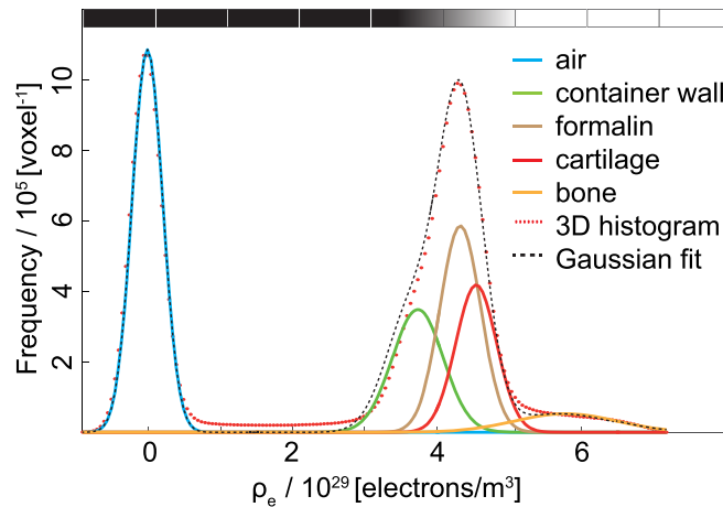
FIG. 5. Histogram of the three-dimensional data from the knee sample measured in the phase-contrast mode with the corresponding multi-Gaussian fit. From the Gaussians related to the constituents, the electron densities of air, container, formalin, cartilage, and bone can be reasonably determined.
