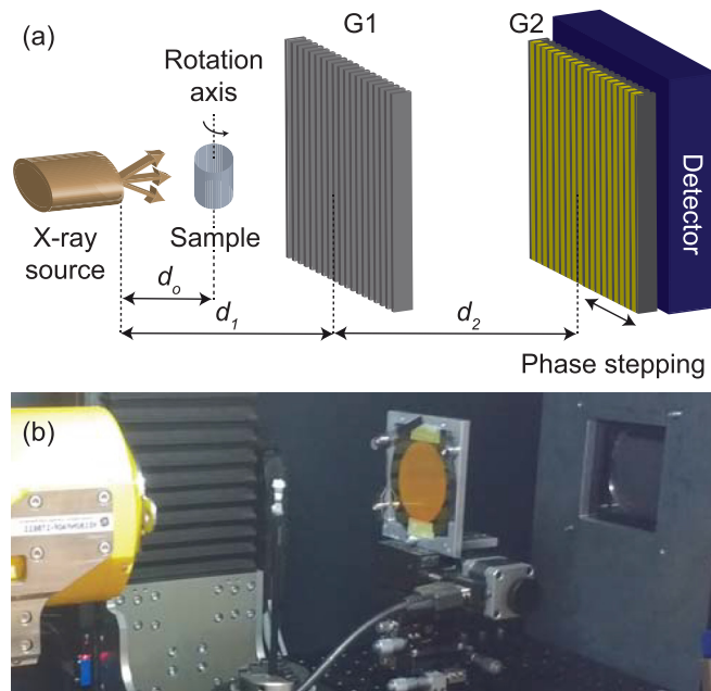
FIG. 1. (a) Scheme and (b) realization within the \mu CT system nanotom ® m of a double-grating symmetric ( d_1 = d_2 ) interferometric set-up. G1: phase grating; G2: analyzer grating; d_0 : distance from the source to the sample; d_1 : distance from the source to phase grating G1; d_2 : distance from the phase grating G1 to analyzer grating G2.
