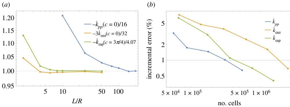
Figure 4. Numerical convergence of the hydrodynamic coefficients in (3.13) for a circular shell. (a) Convergence with respect to the size L of the bounding box \mathcal{S} ; \hat{k}_{pp}(c=0) and k_{\alpha\alpha}(c=0) have been scaled with respect to their analytical values, while \hat{k}_{\alpha\varphi} is scaled with respect to its numerical value when L=200R . (b) Convergence with respect to the number of FE cells for L=100R .
