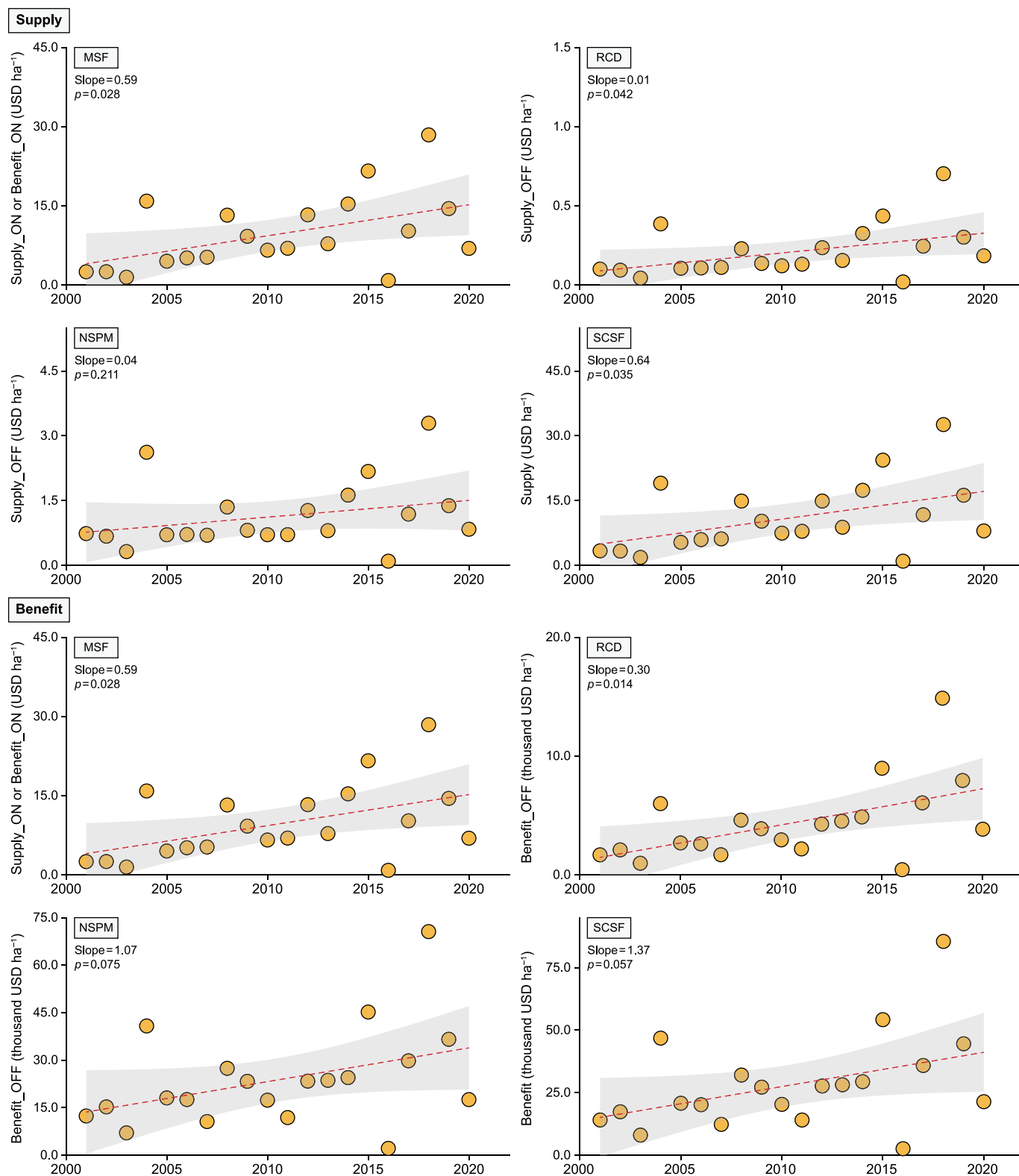
Fig. 2. Evolution of supply and benefit values over time for various Yellow River Basin (YRB) services. MSF: maintenance of soil fertility, RCD: reduction of dredging project costs, NSPM: nonpoint source pollution mitigation, SCSF: total supply values of various services. Please refer to Figs. S4 and S5 in the Supplementary Materials for upstream, midstream, and downstream change trends. The shaded part of the figure represents the 95% confidence interval.
