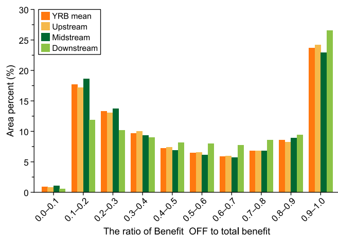
Fig. 3. Ratio of off-site service benefit (Benefit_OFF) to the total service benefit values across the entire Yellow River Basin (YRB) and various regions within the basin. YRB mean, Upstream, Midstream, and Downstream signify the respective overall area percentages of the YRB, the upstream region, the midstream region, and the downstream region, respectively. For a detailed breakdown of the spatial division, please refer to Fig. S1 in the Supplementary Materials.
