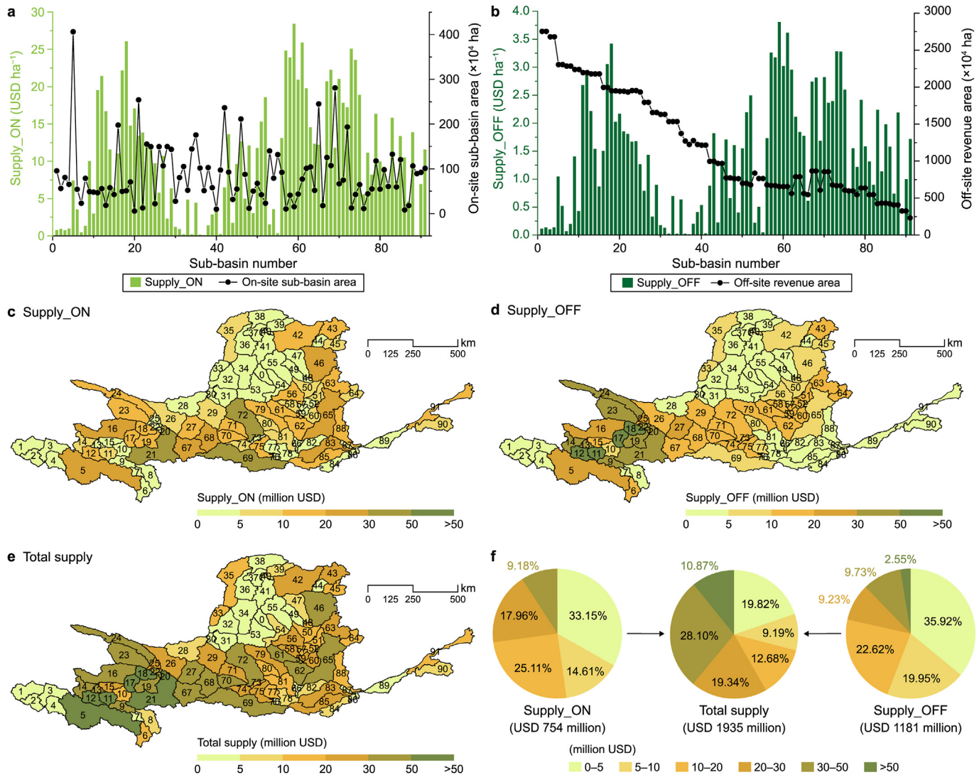
Fig. 4. a–b, Spatial ranking of on-site supply, off-site supply, and total supply values in the Yellow River Basin (YRB). Panels show the multi-year average of on-site (Supply_ON, a) and off-site (Supply_OFF, b) service supply per unit area in different sub-basins and corresponding sub-basin (a) and sub-basin revenue (b) areas. c–e, The on-site (Supply_ON, c), off-site (Supply_OFF, d), and total (e) service supply spatial ranking (in million USD). f, The proportion of different range values in on-site (Supply_ON), off-site (Supply_OFF), and total service supply. The middle number in the pie chart is the total value of the YRB under each supply type.
