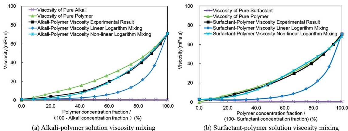
Fig. 6 Alkali-surfactant-polymer multi-component viscosity mixing calculation methods.
