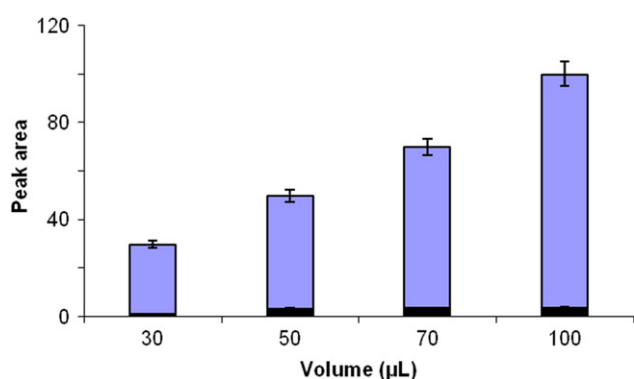
Figure 2 Effect of volume of ionic liquid on the extraction of amitriptyline. Experimental conditions are as follows: aqueous sample volume 5 mL concentration level at 1 \mu\text{g}/\text{mL} ; sample pH 11; 480 rpm stirring rate; 5 min extraction time and 2.5 \mu\text{L} injection volume.
