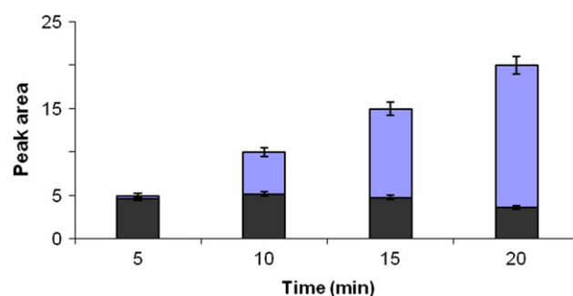
Figure 4 Effect of extraction time on the peak area of amitriptyline. Experimental conditions are as follows: aqueous sample volume 5 mL concentration level at 1 \mu\text{g}/\text{mL} ; sample pH 11; 100 \mu\text{L} [\text{C}_6\text{MIM}][\text{PF}_6] ; 720 rpm stirring rate and 2.5 \mu\text{L} injection volume.
