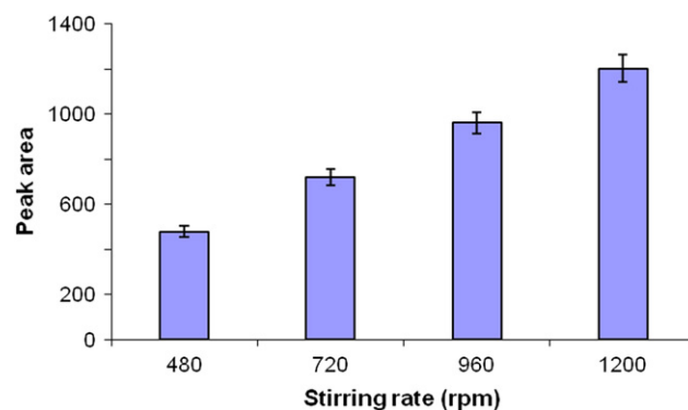
Figure 3 Effect of stirring rate on the extraction of amitriptyline. Experimental conditions are as follows: aqueous sample volume 5 mL concentration level at 1 \mu\text{g}/\text{mL} ; sample pH 11; 100 \mu\text{L} [\text{C}_6\text{MIM}][\text{PF}_6] ; 5 min extraction time and 2.5 \mu\text{L} injection volume.
