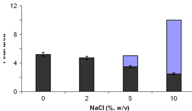
Figure 5 Effect of addition of NaCl on extraction efficiency. Experimental conditions are: aqueous sample volume 5 mL concentration level at 1 µg/mL; sample pH 11; 100 µL [C 6 MIM][PF 6 ]; 720 rpm stirring rate; extraction time 10 min and 2.5 µL injection volume.
