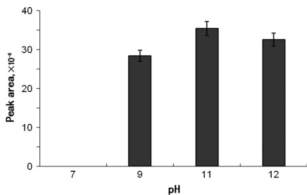
Figure 1 Effect of aqueous solution pH on the extraction of analyte into the drop. Experimental conditions are as follows: aqueous sample volume 5 mL concentration level at 1 \mu\text{g}/\text{mL} ; 100 \mu\text{L} [\text{C}_6\text{MIM}][\text{PF}_6] ; 480 rpm stirring rate; 5 min extraction time and 2.5 \mu\text{L} injection volume.
