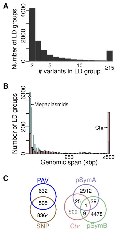
FIG 1 (A) Distribution of number of variants per LD group (at r^2 \geq 0.95 ), (B) distribution of genomic distance spanned by LD groups found on the chromosome or the megaplasmiids (including only groups found only on one replicon), and (C) number of groups containing only PAVs, only SNPs, or both as well as the number of LD groups found within and across replicons. There were 22,057 SNPs and 10,674 PAVs that were not grouped with other variants and 9,501 LD groups with a median of three variants per group, and the largest group contained 6,970 variants. Half of all variants are in groups that contain \leq 12 variants. Only variants used for association testing (minor allele frequency \geq 5\% , missingness \leq 20\% ) were grouped.
