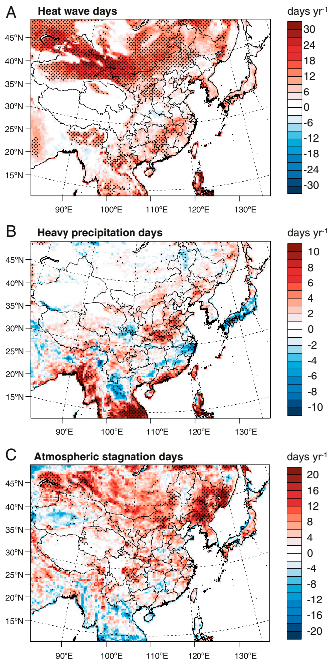
Fig. 3. Projected multiyear mean changes in the frequency of extreme events over East Asia. Projected changes in the frequency of heat wave days (A), heavy precipitation days (B), and atmospheric stagnation days (C) over East Asia are shown from current (2006 to 2010) to future (2046 to 2050) years under RCP4.5. The dots denote areas where changes are statistically significant at the 90% level, as determined by a Student's 2-sample t test.
