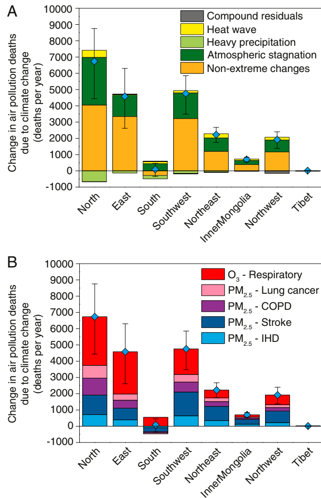
Fig. 4. Climate-induced air pollution-related mortality according to climate mechanism and cause in the 8 regions of China. Changes in air pollution deaths related to climate change under RCP4.5 are shown from current (2006 to 2010) to future (2046 to 2050) years in different regions of China, according to climate mechanism (A) and cause of death (B). The total climate-induced air pollution-related mortality is plotted as blue diamonds. Error bars denote 95% CIs, determined by uncertainties in the RRs. (A) Climate mechanisms are changes in mean climate state (excluding extremes, nonextreme changes), extreme-induced additional changes from heat waves, heavy precipitation, atmospheric stagnation, and the residuals due to compound extremes. (B) Causes are respiratory disease, lung cancer, COPD, stroke, and IHD.
