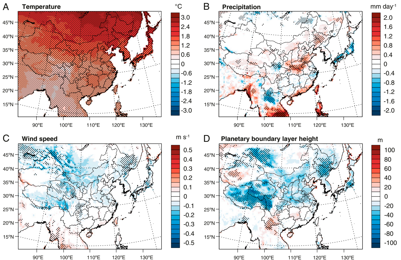
Fig. 1. Projected multiyear mean changes in major meteorological variables over East Asia. Projected mean changes in surface air temperature (A), precipitation (B), surface wind speed (C), and planetary boundary layer height (D) over East Asia are shown from current (2006 to 2010) to future (2046 to 2050) years under RCP4.5. The dots denote areas where changes are statistically significant at the 90% level, as determined by a Student's 2-sample t test.
