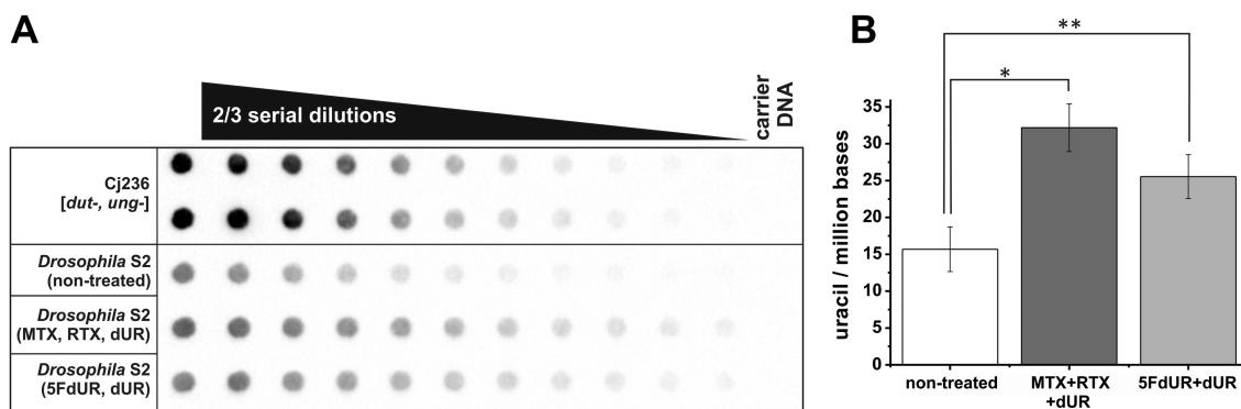
Figure 6. Dot-blot assay for measuring genomic uracil levels of Drosophila Schneider S2 cells after treatment with de novo thymidylate biosynthesis pathway inhibitors. (A) CJ236 [ dut- , ung- ] Escherichia coli genomic DNA was used as standard for the dot-blot assay. Genomic uracil content of different drug-treated (5FdUR, dUR or MTX, RTX, dUR) and non-treated Drosophila S2 cells were measured. (B) Bar graph shows the uracil moieties/million bases of each sample (mean values \pm the standard errors of the mean). Both types of treatments led to significantly elevated genomic uracil levels as compared to non-treated cells (* = P < 0.01 , ** = P < 0.05 ). Calculations were based on six independent datasets ( n = 6 ).
