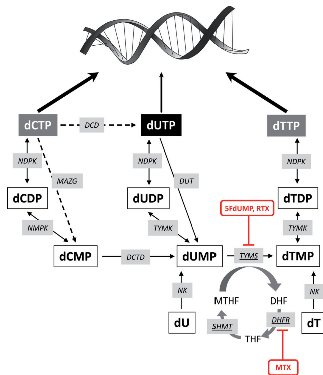
Figure 4. Pathways involved in thymidine synthesis in Escherichia coli , Drosophila melanogaster and humans. Key steps in dNTP synthesis focusing on the de novo thymidylate biosynthesis are shown (directly involved enzymes underlined). Dashed arrow shows pathways only present in E. coli . Inhibitors of the pathway are shown in red. 5FdUMP (5-fluorodeoxyuridylylate), the metabolite of 5FU and 5FdUR, along with raltitrexed (RTX) inhibits thymidylate synthase (TYMS) while methotrexate (MTX) inhibits dihydrofolate reductase (DHFR). The enzyme responsible for dCTP-dCMP conversion in mammals is DCTPPI (dCTP pyrophosphatase 1) (78), however, using a BLAST search, no clearcut homologue could be identified in D. melanogaster , hence we did not include it in this Figure. In E. coli , the nucleoside triphosphate pyrophosphohydrolase MAZG is responsible for this activity (79). Abbreviations are as follows: DCD: dCTP deaminase, DCTD: dCMP deaminase, DUT: dUTPase, DHF: dihydrofolate, DHFR: dihydrofolate reductase, MTHF: 5,10-methylene tetrahydrofolate, NDPK: nucleoside-diphosphate kinase, NK: nucleoside kinase, MAZG: nucleoside triphosphate pyrophosphohydrolase, NMPK: nucleoside monophosphate kinase, SHMT: serine hydroxymethyltransferase, THF: tetrahydrofolate, TYMK: dTMP kinase, TYMS: thymidylate synthase.
