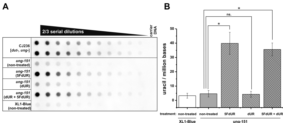
Figure 5. Dot-blot assay for measuring genomic uracil levels of 5FdUR, dUR treated Escherichia coli cells. (A) CJ236 [ dut- , ung- ] E. coli genomic DNA was used as standard for the dot-blot assay. Quantity of genomic uracil of different drug-treated (5FdUR and dUR or both) and non-treated E. coli BL21(DE3) ung-151 samples were measured along with XL1-Blue [ dut+ , ung+ ], applied as a negative control. (B) Bar graph shows the uracil moieties/million bases of each sample (mean values \pm the standard errors of the mean). Significant increase (*) in uracil-DNA content was only observed using 5FdUR treatment, or the combined 5FdUR and dUR treatment as compared to non-treated cells ( P < 0.05 ). Calculations were based on six independent datasets ( n = 6 ).
