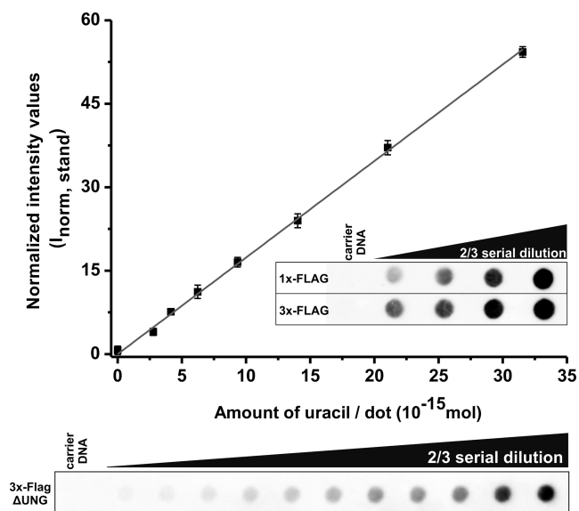
Figure 3. Design of a standard curve for in vitro quantification of genomic uracil levels. Genomic DNA isolated from log phase growing CJ236 [ dut - , ung - ] Escherichia coli strain was used as a standard with well-defined uracil-content during quantification. Applying a serial dilution of this standard provides a wide and reproducible range for uracil quantification. The normalized calibration curve is from four independent datasets ( n = 4 ), where error bars show standard errors of the mean (SEM). The inset shows that the 3 \times FLAG- \Delta UNG construct is slightly more sensitive under similar conditions, compared to the 1 \times FLAG- \Delta UNG construct (as based on a 4 point two-third serial dilution, starting with 100 ng of standard genomic DNA).
