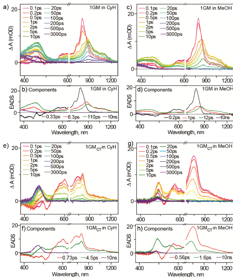
Figure 3. Time evolution of the transient absorption spectra of (a) 1GM in cyclohexane, (c) 1GM in methanol, (e) 1GM CT in cyclohexane, and (g) 1GM CT in methanol. The corresponding evolution-associated difference spectra (EADS) are shown in panels (b, d, f, h), respectively. The “10 ns” component represents a long-lived product state with an arbitrarily long lifetime beyond the maximum pump-probe delay time.
