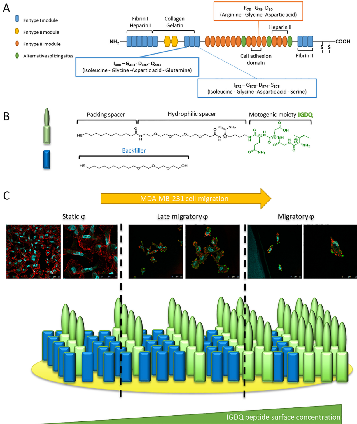
Fig. 1. Peptide-associated cell migration along engineered surfaces. A. Schematic representation of fibronectin and its functional motifs; B: Chemical structure of the peptides used for the gradient with the fibronectin motif IGDQ and the tetraethylenglycol as backfiller; C: Schematic representation of engineered surfaces after 5 days of cell migration; Immunofluorescent confocal microscopy images from control MDA-MB-231 cells (shCTL) labeled for ITGB3 (green), cytoskeleton (phalloidin – alpha-tubulin – red) and nucleus (Hoechst – UV / blue); \phi : phenotype; static: proliferative cells; late migratory: cells which start migrating after day 3 of the experiment; migratory: cells which start migrating before day 3 of the experiment.
