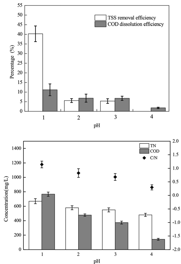
Fig. 1 Sludge disintegration efficiency under different pH values (the dosage of \text{NaNO}_2 was 0.3 \text{ g g}^{-1} TSS at room temperature ( 25 \text{ }^\circ\text{C} )).
