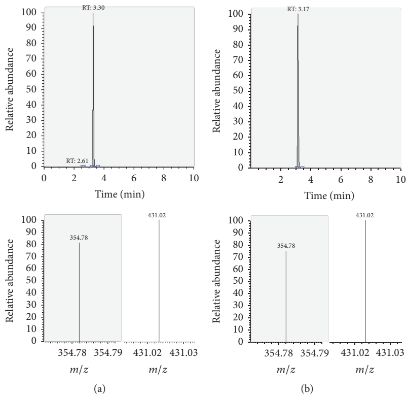
FIGURE 11: LC-MS/MS chromatograms of FLA and SRM transitions and relative abundances. (a) Standard in a 100 µg L -1 solution. (b) Standard in the spiked sample at 100 mg kg -1 .
