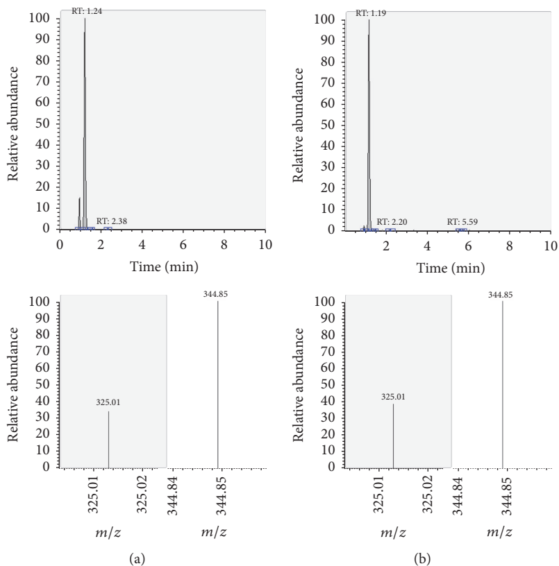
FIGURE 6: LC-MS/MS chromatograms of TRM and SRM transitions and relative abundances. (a) Standard in a 100 µg L -1 solution. (b) Standard in the spiked sample at 100 mg kg -1 .
