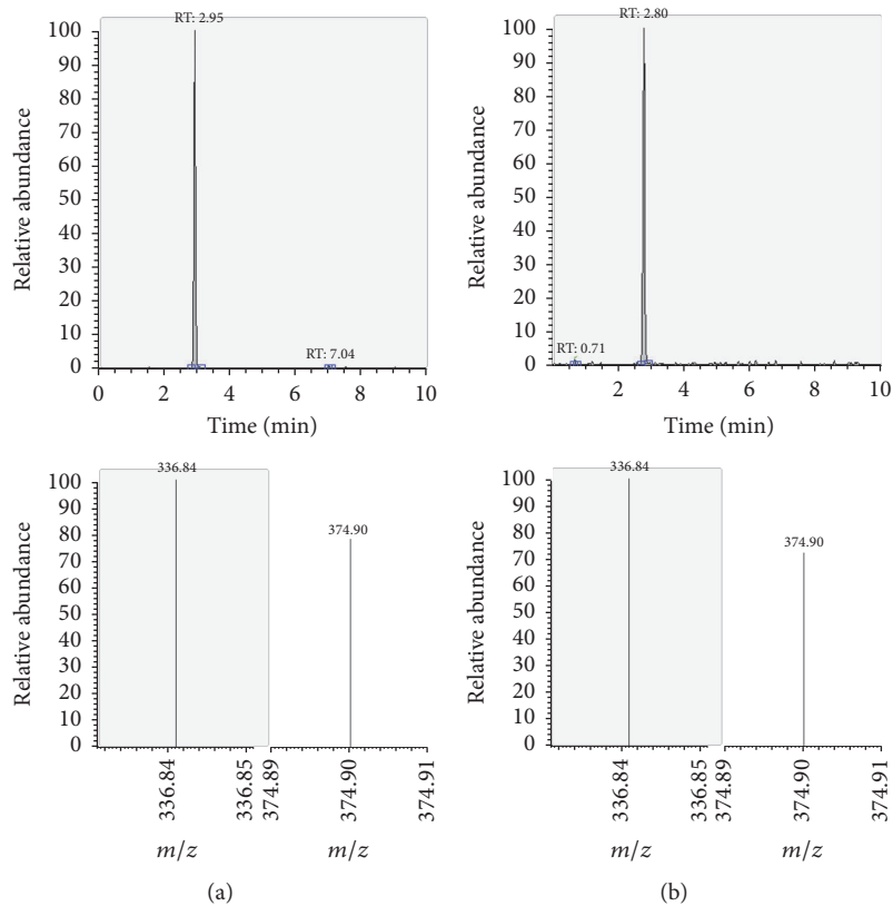
FIGURE 10: LC-MS/MS chromatograms of TRA and SRM transitions and relative abundances. (a) Standard in a 100 µg L -1 solution. (b) Standard in the spiked sample at 100 mg kg -1 .
