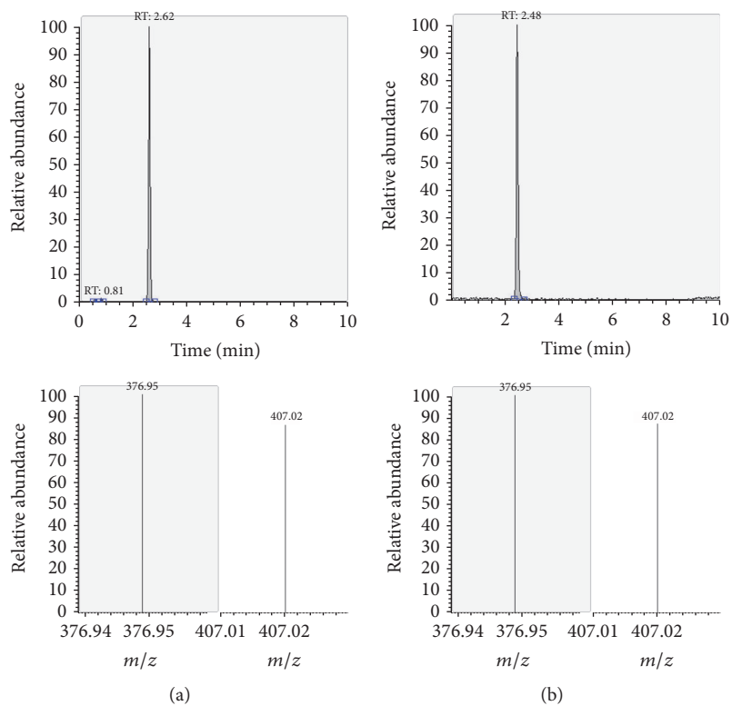
FIGURE 7: LC-MS/MS chromatograms of BCL and SRM transitions and relative abundances. (a) Standard in a 100 µg L -1 solution. (b) Standard in the spiked sample at 100 mg kg -1 .
