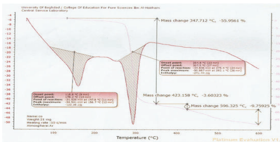
FIGURE 5: TG/DTG and DSC thermogram of [\text{Co}(\text{L}^1)(\text{L}^2) \text{H}_2\text{OCl}] in argon atmosphere.
