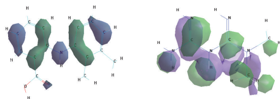
FIGURE 1: HOMO-LUMO categories of the ligands (mefenamic acid and metformin).
