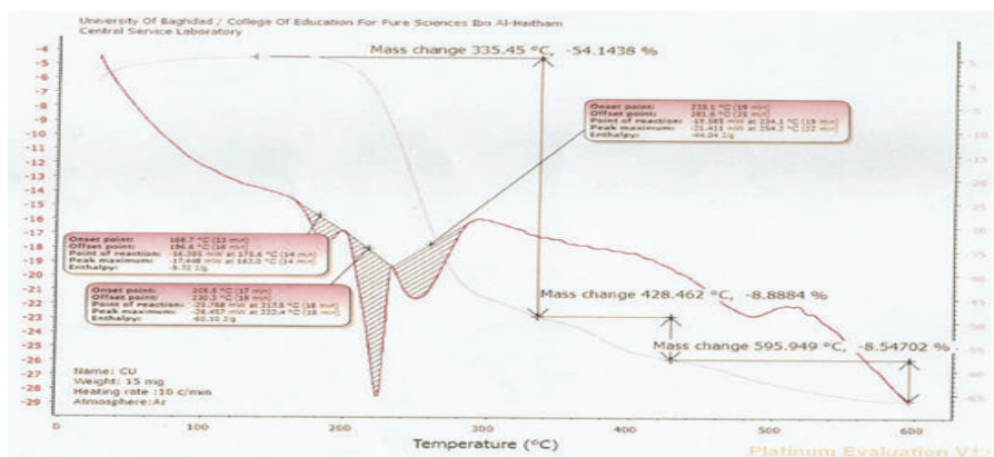
FIGURE 6: TG/DTG and DSC thermogram of [\text{Cu}(\text{L}^1)(\text{L}^2) \text{H}_2\text{OCl}] in argon atmosphere biological activity.
