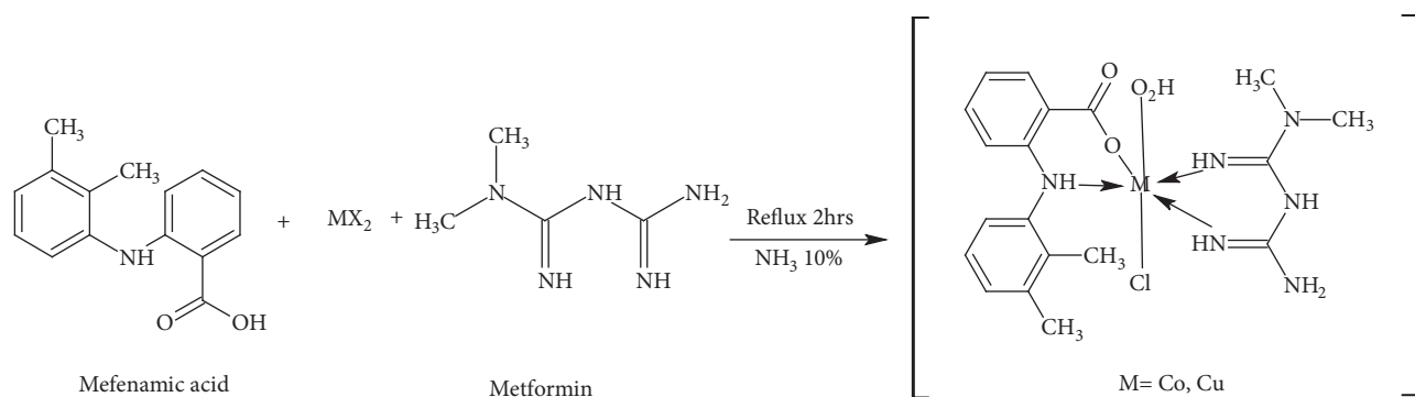
SCHEME 1: Synthesis of mixed drug complexes.
