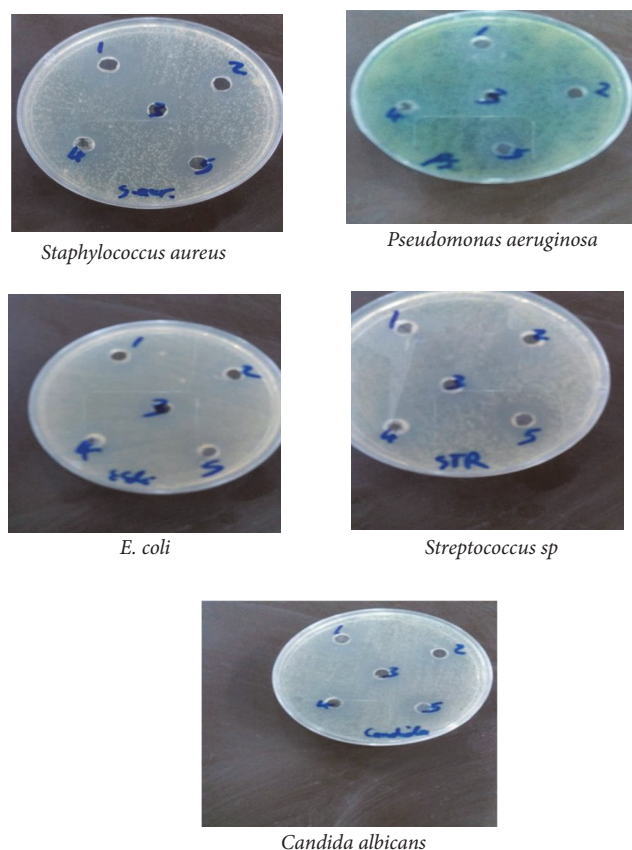
FIGURE 7: Effect of ligands and their complexes in the inhibition of different kinds of bacteria.
