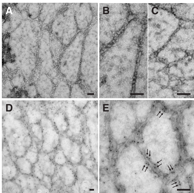
Figure 3 MBP-ZP-N-6his assembles into filaments. (A-C) Electron micrographs showing overview (A) and details (B, C) of negatively stained samples. (D, E) Immunogold localisation using monoclonal anti-MBP. Arrows mark closely spaced pairs of beads. Bars represent 0.1 \mu\text{m} .
