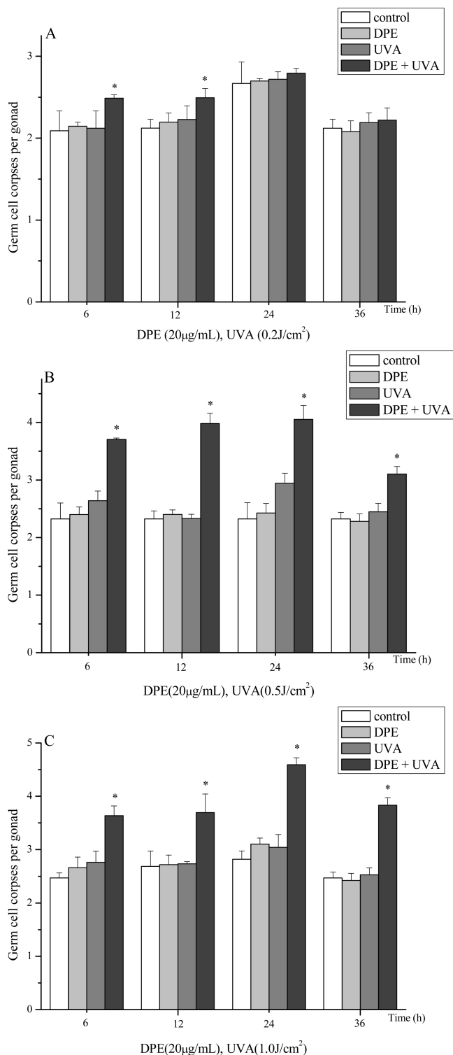
Figure 3. Time course of germ cell death in C. elegans induced by 20 \mu\text{g}/\text{mL} DPE + 0.2 \text{J}/\text{cm}^2 UVA (A), 20 \mu\text{g}/\text{mL} DPE + 0.5 \text{J}/\text{cm}^2 UVA (B), and 20 \mu\text{g}/\text{mL} DPE + 1.0 \text{J}/\text{cm}^2 UVA (C). Synchronized young adult hermaphrodites were exposed to DPE, UVA, or DPE + UVA, and germ cell corpses were scored at time points of 6, 12, 24, and 36 h, respectively. Data are pooled from three independent experiments. All values are presented as the means \pm SE; n \geq 20 , and * represents P < 0.05 .
