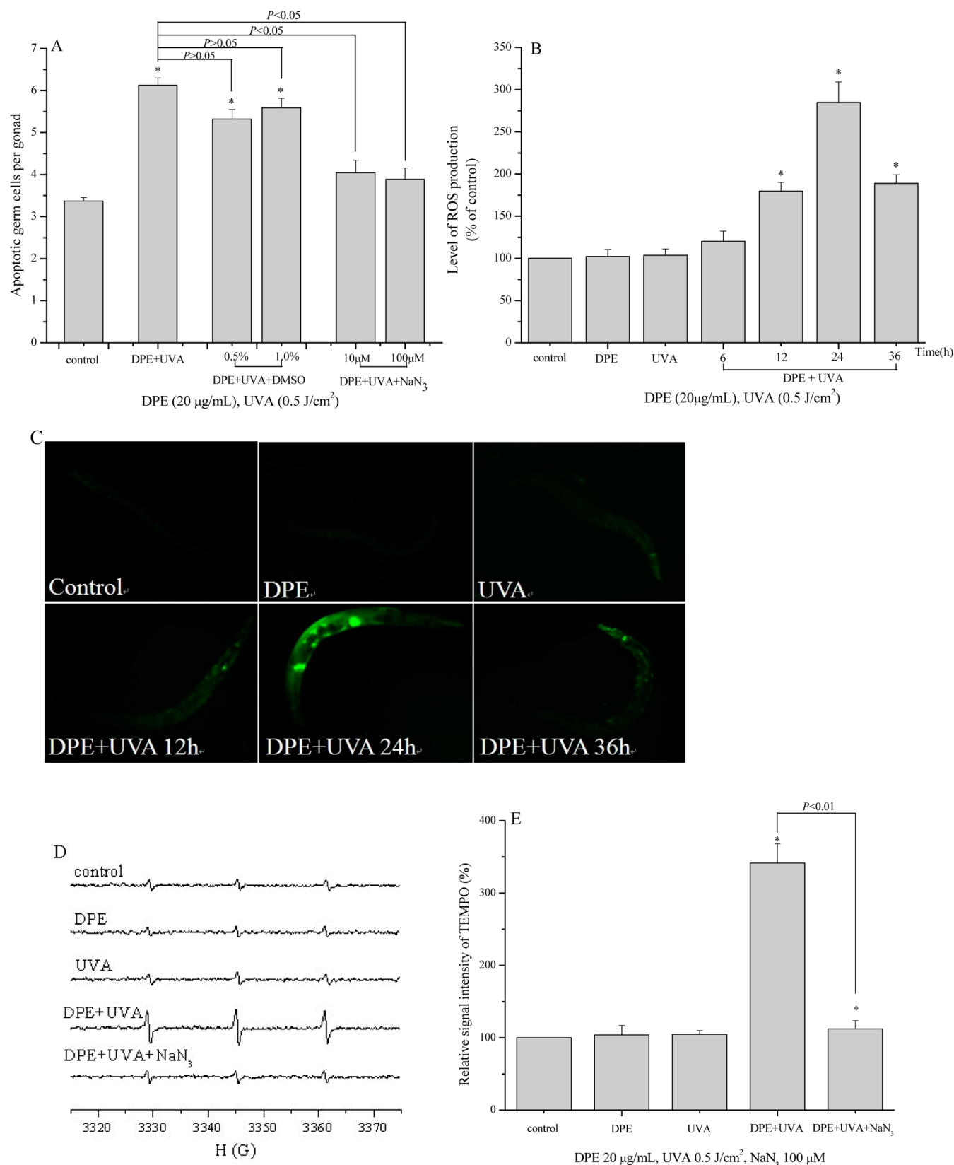
Figure 8. ROS, especially ^1\text{O}_2 , play a crucial role in germ cell apoptosis induced by DPE ( 20\ \mu\text{g/mL} ) plus UVA ( 0.5\ \text{J/cm}^2 ). (A) The induction of germ cell apoptosis by DPE plus UVA was effectively rescued by \text{NaN}_3 , a specific ^1\text{O}_2 scavenger. (B) The in situ expression of fluorescence was measured using DCF-DA (a molecular probe) in single whole worms. (C) The relative fluorescence was determined using Image-Pro Plus, version 6.0. (D) Three-line ESR spectra of the 4-O-TEMPO signal. (E) Relative signal intensity of 4-O-TEMPO. All these results suggested that ROS, especially ^1\text{O}_2 , play a pivotal role in the induction of germ cell apoptosis by DPE plus UVA. Data were pooled from at least three independent experiments. All values are presented as the means \pm SE; n \geq 40 , and * represents P < 0.05 .
