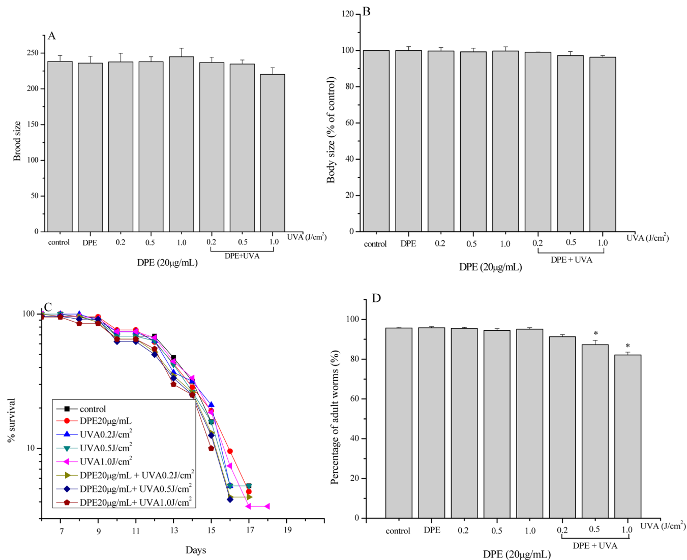
Figure 5. Effects of DPE plus UVA on the worms' development. (A) Age-synchronized young hermaphrodites were treated with either DPE (20 \mu\text{g}/\text{mL} ) or UVA (0.2–1.0 \text{J}/\text{cm}^2 ) alone or in combination (DPE + UVA) for 24 h at 20 ^{\circ}\text{C} , then the brood size was counted. (B) The body sizes were determined by measuring the flat surface area of the worms using ImageJ software, and there was no difference among all treatments after L1-stage larvae were treated with DPE and/or UVA for 72 h. (C) Life span curves of worms and (D) the percentage of adult worms were scored after L1-stage larvae were treated with DPE and/or UVA for 72 h. Data were pooled from three independent experiments. All values are presented as the means \pm SE; n \geq 20 , and * represents P < 0.05 .
