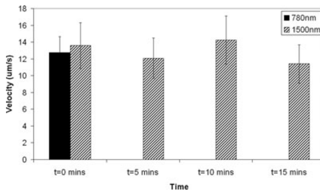
Fig. 4. Cytoplasmic organelle streaming velocities in Spirogyra from t = 0 min to t = 15 min were measured from movies taken at 5 min intervals after irradiation with the \lambda = 780 nm Ti:Sapphire or bi-directionally pumped OPO at \lambda = 1500 nm ( n = 5 cells per time interval for each laser).
