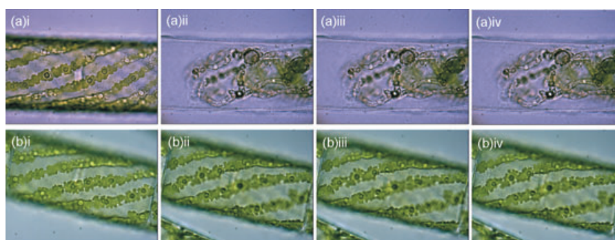
Fig. 3. (a) Brightfield images of Spirogyra taken after constant irradiation with the femtosecond-pulsed \lambda = 780 nm Ti:Sapphire laser for time periods of (i) t = 0 min, (ii) t = 5 min, (iii) t = 10 min and (iv) t = 15 min. (b) shows brightfield images for the same irradiation times using the femtosecond-pulsed bi-directionally pumped OPO at \lambda = 1500 nm. The difference in colour is merely due to a different white balance setting of the camera.
