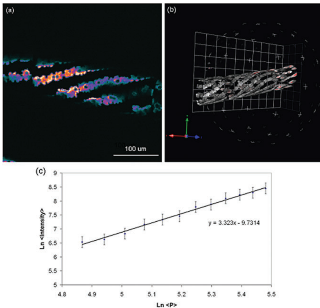
Fig. 2. (a) A pseudo-colour cross-sectional auto-fluorescence image of Spirogyra taken using the bi-directional pumped OPO at \lambda = 1500 nm, and with an average power of 31 mW at the specimen. The bright bands with serrated edges are optical cross sections of the chloroplasts. The dark circular spots visible at intervals along the chloroplasts are pyrenoids (carbohydrate reserve granules characteristic of this genus of alga). (b) Three-dimensional auto-fluorescence reconstruction of Spirogyra using a 'red hot' look-up table (volocity, improvisation). The unit cell of the grid is 28.03 \mu\text{m} . (c) Log-log plot with a gradient of 3.3 confirms the three-photon nature of the auto-fluorescence excitation.
