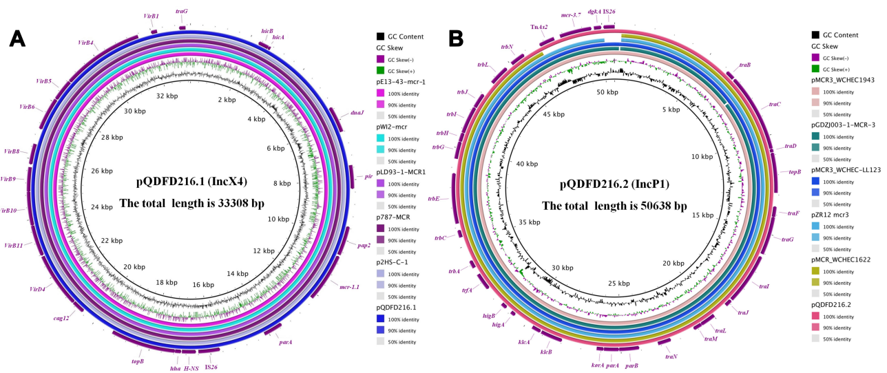
Figure 1 Comparison of mcr -carrying plasmids and other closely related plasmids. (A) Comparative analysis of pQDFD216.1 with five closely related mcr-1.1 -carrying plasmids including pLD93-1-MCR1 (GenBank accession: CP047664.1), p2HS-C-1 (GenBank accession: CP038181.1), p787-MCR (GenBank accession: MG825367.1), pE13-43- mcr-1 (GenBank accession: LT838201.1) and pW12- mcr (GenBank accession: LT838201.1). pQDFD216.1 was used as the reference plasmid for BRIG. (B) Comparative analysis of pQDFD216.2 with five closely related mcr-3 -carrying plasmids, pMCR3_WCHEC1943 (GenBank accession: MF678351.1), pGDZJ003-1-MCR-3 (GenBank accession: MH043625.1), pMCR3_WCHEC-LL123 (GenBank accession: MF489760.1), pZR12 (GenBank accession: MF455227.1) and pMCR_WCHEC1622 (GenBank accession: KY463452.1). The plasmid pQDFD216.2 was used as the reference plasmid for BRIG.
