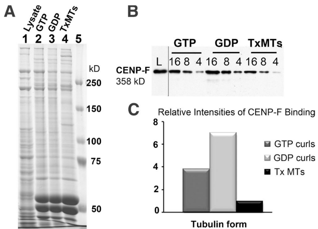
Figure 3. Tubulin curls made with either GTP or GDP will pull down CENP-F better than Tx-MTs. (A) RPE1 cells were synchronized, collected, and extracted as described in Materials and methods, and then mixed with either vinblastine-induced tubulin curls or Tx-MTs and pelleted. A 4x pellet volume of cell extract and equal volumes of each pellet were fractionated on 7% polyacrylamide gels. 1, cell lysate; 2, 3, and 4, pellets of GTP curls, GDP curls, and Tx-MTs, respectively; 5, molecular mass markers. (B) The gels from A blotted to nitrocellulose paper and reacted with a mouse monoclonal antibody to CENP-F (Santa Cruz Biotechnology, Inc.). Numbers above blot lanes indicate the number of microliters loaded. (C) Ratios of curls/Tx-MTs staining, as measured by densitometry. The binding ratios for GTP curls and Tx-MTs shown here are from a single representative experiment out of three repeats.
