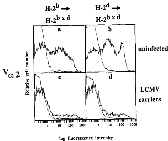
Figure 1. LCMV/H-2D b -specific \alpha/\beta TCR transgenic thymocytes developing in the absence (uninfected; a and b ) or presence (LCMV carriers; c and d ) of the viral antigen. Unseparated thymocytes were stained with mAb B20.1 specific for the transgenic V \alpha 2 chain. Both H-2 b ( c ) and H-2 d ( d ) bone marrow-reconstituted (C57BL/6 \times BALB/c) F1 chimeras carrying the LCMV-virus deleted transgenic V \alpha 2 + cells at an early stage of differentiation. Comparable histograms were obtained from stainings with KJ16 specific for the transgenic \beta chain (data not shown). Broken lines indicate control thymocytes stained with fluorescein-conjugated goat anti-rat antibodies alone. Comparable results were obtained from at least four individual chimeras per group. We have been unable to explain the reproducibly higher amount of TCR hi cells in group b as compared with a .
