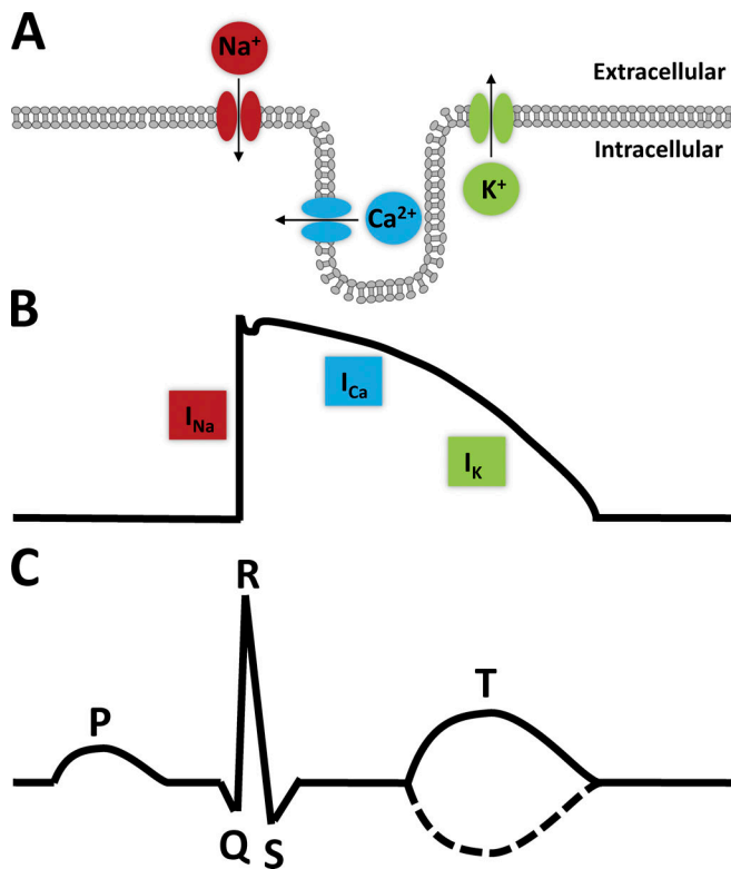
Figure 1. Cardiac electrical activity. (A) Several ionic channels are present on the sarcolemma of cardiac myocytes: Na + , Ca 2+ , and K + channels. Ca 2+ channels are mainly located in transverse tubules when present. Specific ionic channels composition depends on the species and the region of the heart (e.g., atria versus ventricle). (B) Opening and closing of ionic channels are responsible for the action potential. (C) At the body level, surface ECG reflects the electrical activity in the entire heart. P wave is the atrial depolarization, QRS is the ventricular depolarization, and T wave is the ventricular repolarization. In some cases, T wave can be negative (dashed line).
