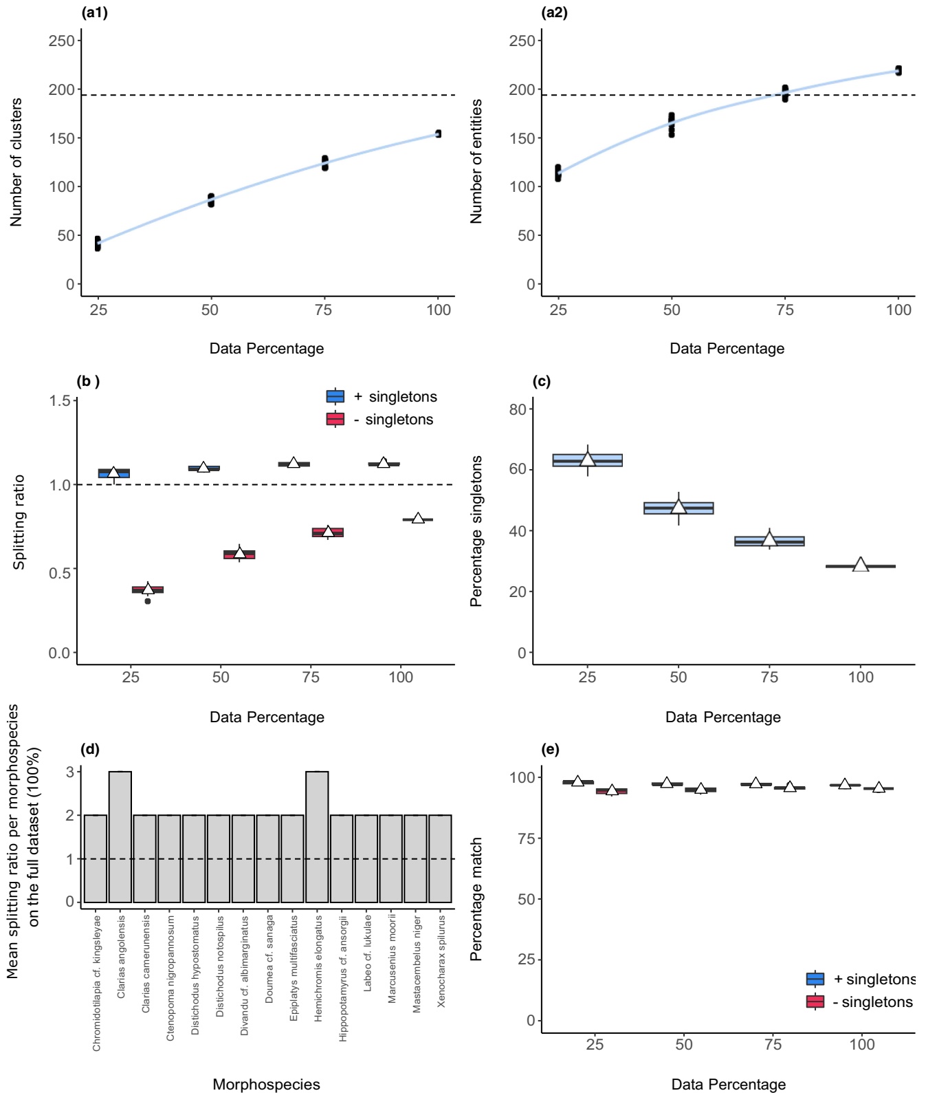
FIGURE 4 SPEDe-sampler results for 741 COI fish sequences. (a1 and a2) The number of clusters and entities across subsetted data set sizes. The light blue band represents a 95% confidence interval. The dotted lines at y = 194 is the number of predefined morphospecies. (b) A boxplot of the splitting ratios across dataset sizes, including (blue) and excluding (red) singletons. The dotted line at y = 1 indicates the expected ratio if no splitting occurred. (c) A boxplot of the percentage of singletons across data set sizes. (d) The mean splitting ratios of morphospecies groups that exceeded a ratio of 1 (dotted horizontal line). (e) A boxplot of the percentage matches between predefined morphospecies and GMYC species, including (blue) and excluding (red) singletons. White triangles represent means
