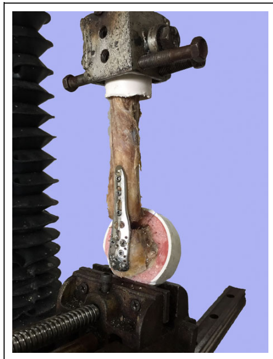
Figure 3. The setting of the axial rotation test.
