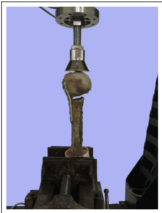
Figure 2. The setting of the varus bending test.
