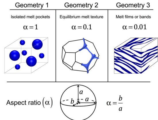
Fig. 2. Conceptual models of the melt geometry used in these calculations. Geometry 1 is based on the studies of Berryman (37, 38). Geometry 2 is modified from Takei (11), Mavko (12), and Schmeling (39). Geometry 3 is modified from Holtzman and coworkers (6, 22). The effect of any intermediate geometry on seismic velocities can be modeled by modifying the aspect ratio ( \alpha ) in Eqs. 3 and 4 [see the study of Takei (11) for further discussion of the derivation of \alpha ].
