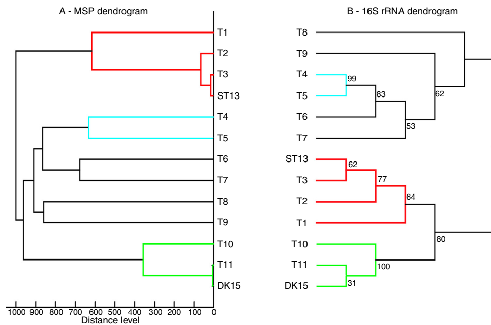
Figure 3 – Comparison between 16S rRNA phylogenetic tree and the MSP dendrogram. A. Mean spectra projection (MSP) dendrogram, B. 16S rRNA based phylogenetic tree of Streptomyces type strains, T1-T11 – DSM type cultures used for grouping of Streptomyces species, T1 - Streptomyces viridis DSM-42078 (T), T2 - S. phaeochromogenes DSM-40788 (T), T3 - S. ederenensis DSM-40741 (T), T4 - S. iakyrus DSM-40482 (T), T5 - S. griseochromogenes DSM-40499 (T), T6 - S. gougerotii DSM-40324 (T), T7 - S. albus DSM-40313 (T), T8 - S. diastaticus DSM-40495 (T), T9 - S. alboflavus DSM-40045 (T), T10 - S. toxytricini DSM-40178 (T), T11 - S. globosus DSM-41122 (T).
