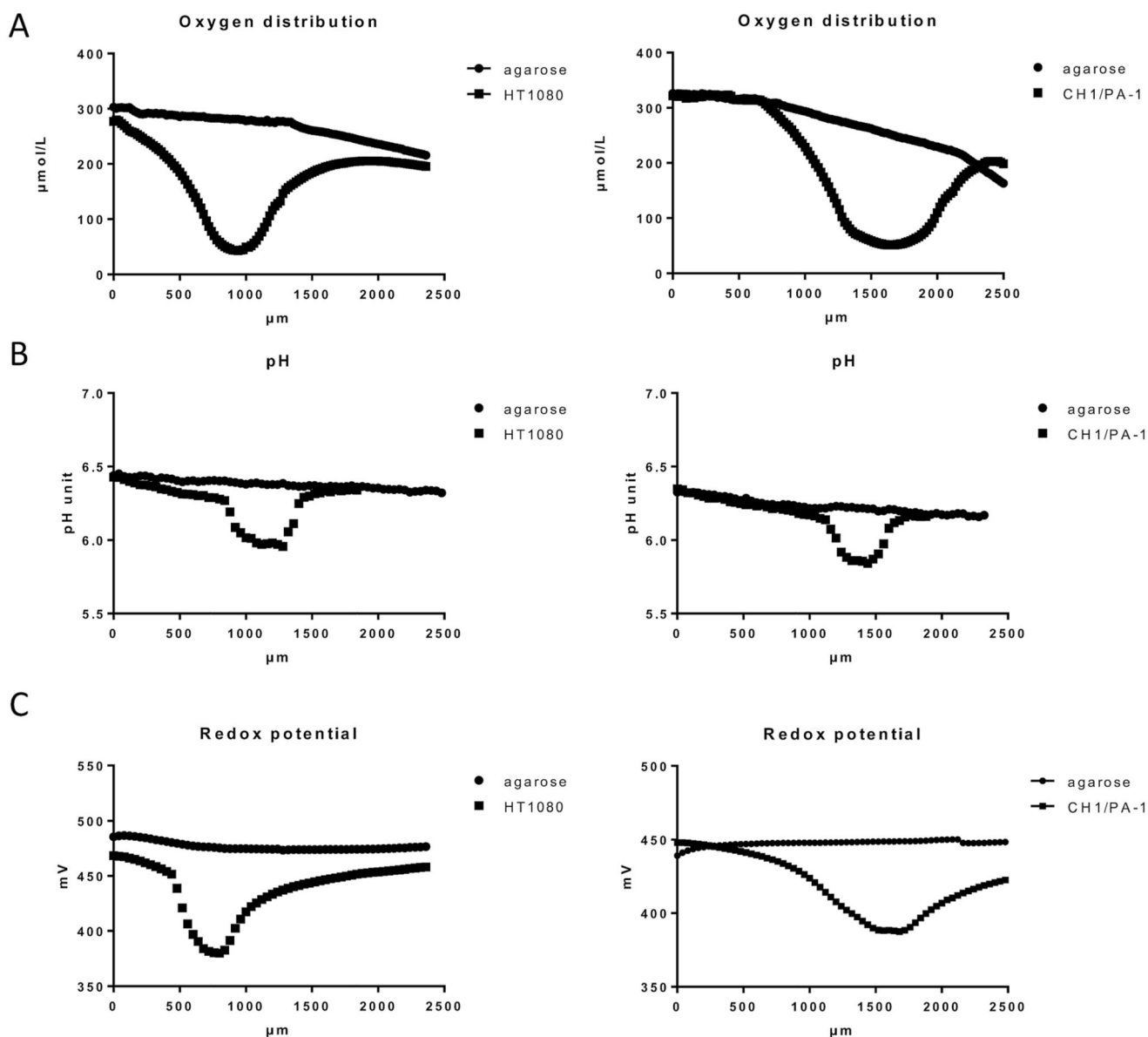
Fig. 2. Physicochemical gradients through agarose-embedded HT1080 and CH1/PA-1 multicellular spheroids (>400 \mu\text{m} diameter) in comparison to agarose medium distant from the spheroid, measured by microelectrodes and exemplified by representative samples. (A) Oxygen distribution (measured in 20 \mu\text{m} intervals), (B) pH (40 \mu\text{m} intervals), (C) redox potential (40 \mu\text{m} intervals). Profile depths are relative to the agarose surface, whereby spheroid location relative to the agarose surface varies.
