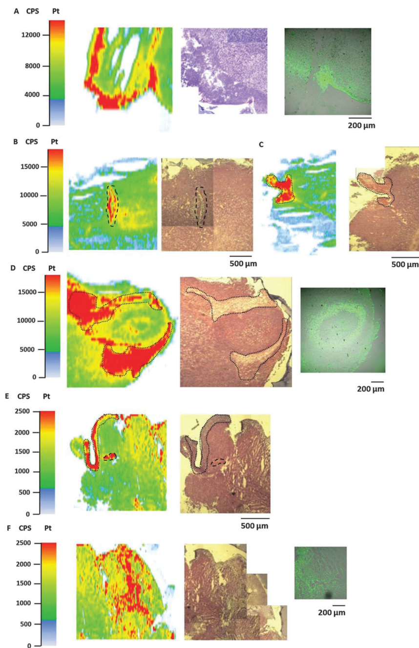
Fig. 6. Platinum distribution in HT1080 tumor sections measured by LA-ICP-MS. Detailed views of ablated tumor samples after treatment with compounds 1 (A), compound 2 (B–D) and satraplatin (E and F); laser platinum image (left), H&E-stained section (middle) and hypoxic regions, visualized by pimonidazole staining (right). The dotted spots in the laser image and H&E-stained slides correspond to loose, connective tissue with sparsely scattered tumor cells. The dashed lines indicate the presence of a blood (micro-)vessel.
