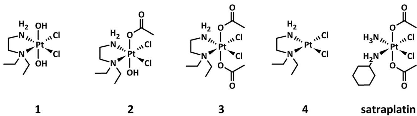
Fig. 1. Chemical structures of the platinum(IV) complexes 1–3 under investigation, including 4 as the main platinum(II) metabolite and the reference compound satraplatin.
