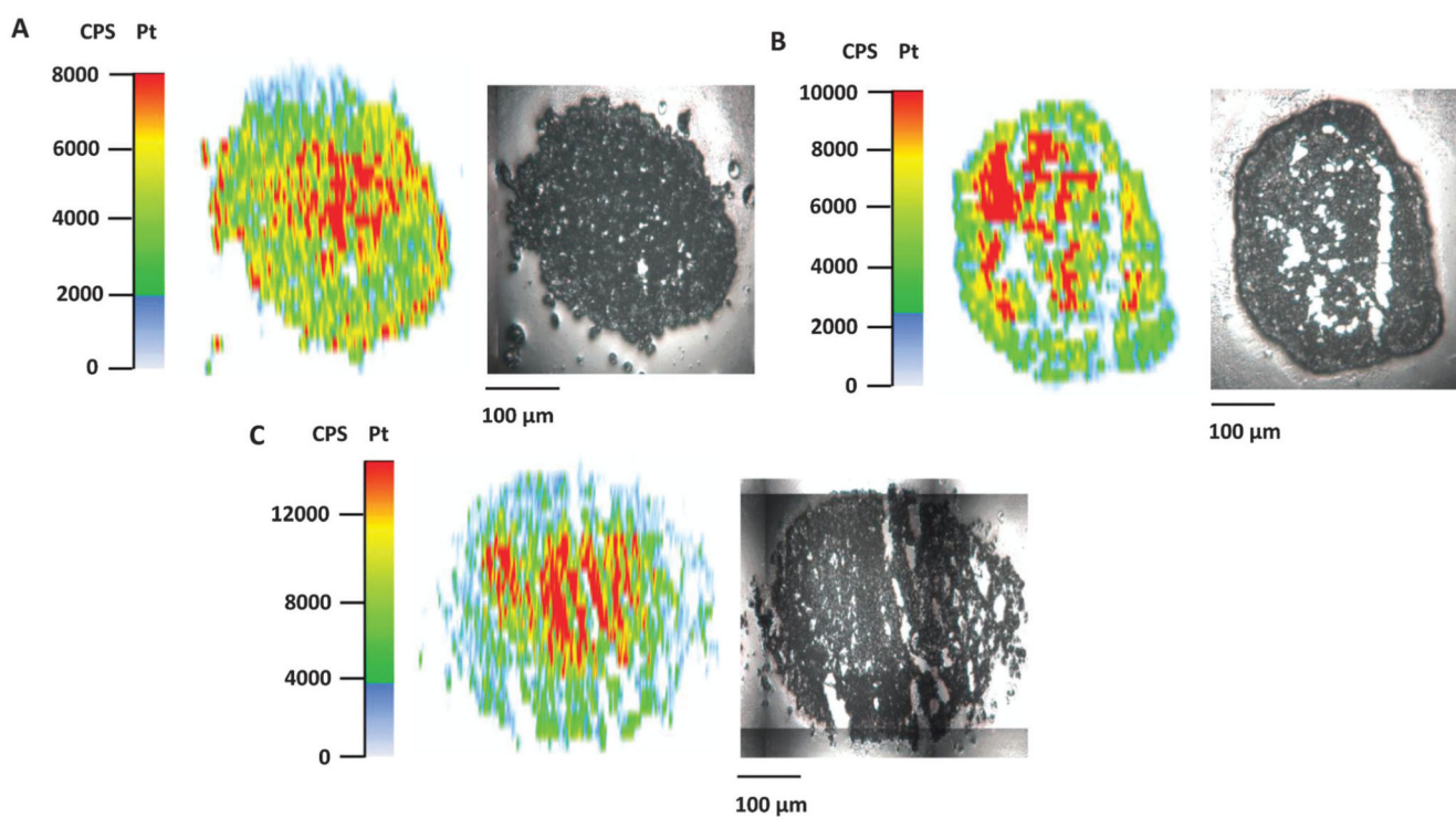
Fig. 4. Platinum distribution in hypoxic HT1080 spheroids upon treatment with (A) compound 1 , (B) compound 2 and (C) satraplatin. Laser ablation-ICP-MS measurements were performed using 20 \mu\text{m} thin cryosections.
