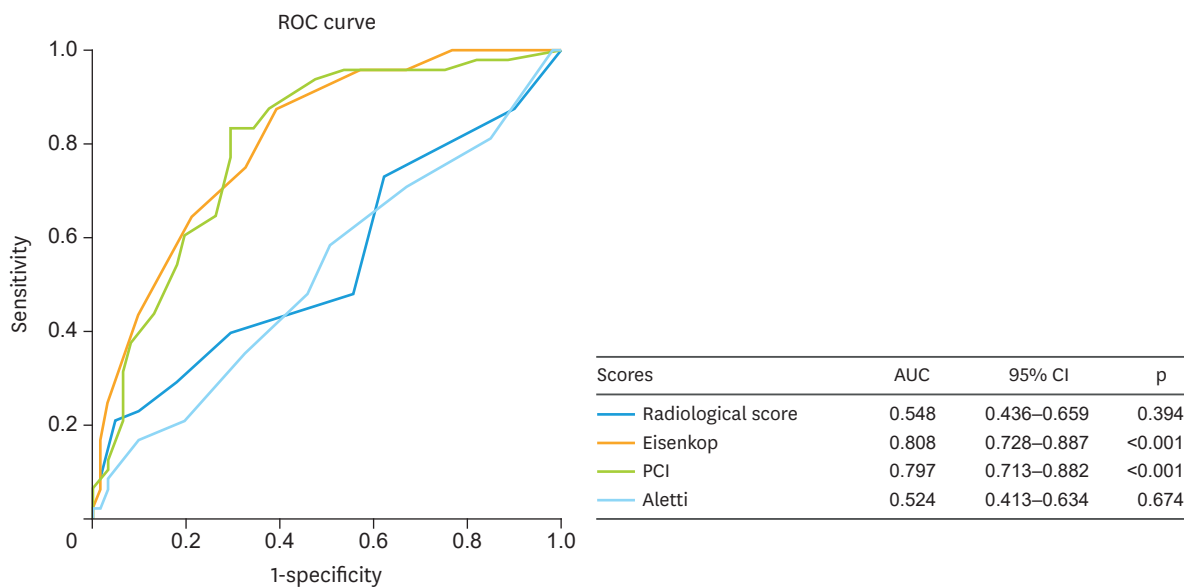
Fig. 2. Discriminatory power of radiological and intraoperative scores for complete resection. AUC, area under the curve; CI, confidence interval; PCI, peritoneal cancer index; ROC, receiver operating characteristics.
