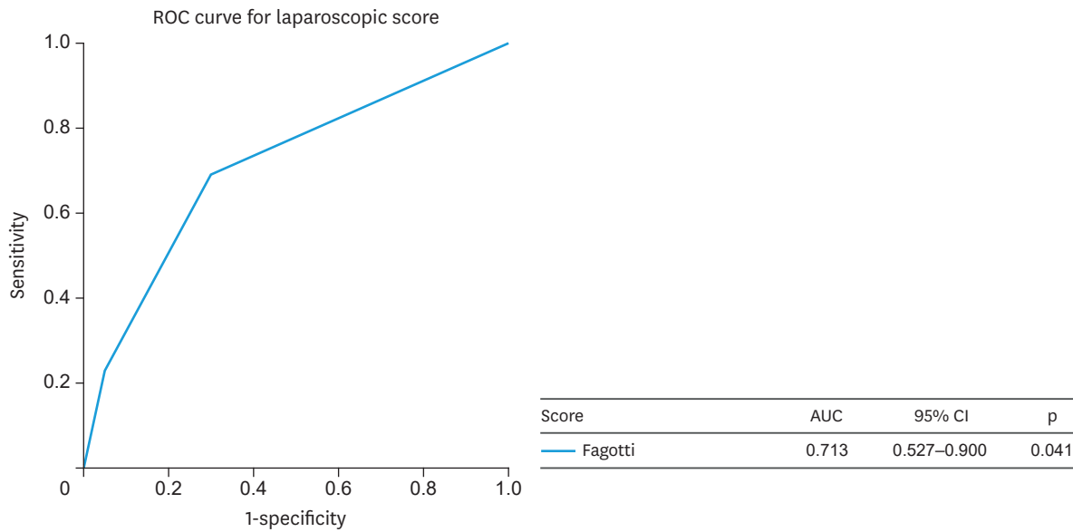
Fig. 3. ROC curve analysis for S-LPS score. AUC, area under the curve; CI, confidence interval; ROC, receiver operating characteristics; S-LPS, staging laparoscopy.
