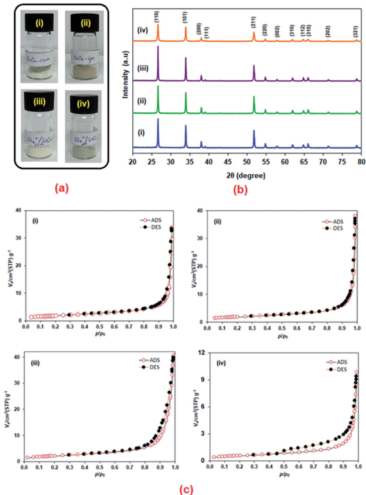
Fig. 3 (a) The colour of the catalyst powders, (b) XRD patterns and (c) N_2 adsorption–desorption isotherms of the (i) SnO_2 -com, (ii) SnO_2 -spc, (iii) sulfonated SnO_2 -com and (iv) sulfonated SnO_2 -spc catalysts.
