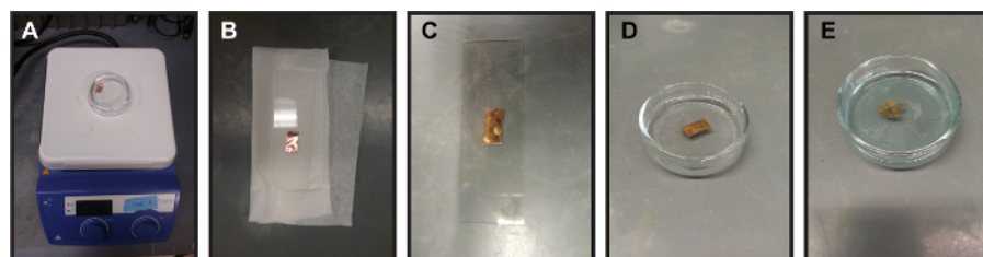
Figure 2. Process for making graphene coated TEM grids (A) Washing the graphene-on-copper piece in warm acetone (B) Removing macroscopic wrinkles by flattening graphene-on-copper between two glass slides. A tissue is placed beneath the graphene-on-copper piece so as to not fold in new wrinkles. (C) Placing amorphous holey carbon TEM grids on graphene-on-copper with amorphous carbon side of TEM grids touching the graphene. (D) Floating copper/graphene/TEM grids on sodium persulfate etchant. This removes the copper from the grids. (E) Graphene coated TEM grids after etching off copper. The solution is blue and there is no copper left on the graphene-coated grids. For size reference, the diameter of the glass Petri dish is approximately 6 cm and the glass slide is 7.5 cm by 2.5 cm. Please click here to view a larger version of this figure.
