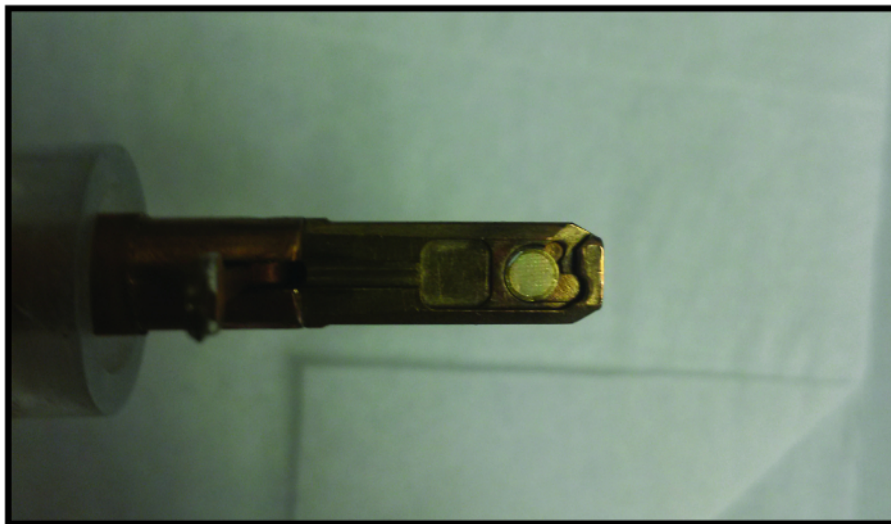
Figure 4. Loading graphene liquid cell into standard single tilt TEM holder. The graphene liquid cell fits in a standard single-tilt TEM holder in the same way a normal TEM grid fits in the holder. For size reference, the TEM grid has a diameter of 3 mm. Please click here to view a larger version of this figure.
