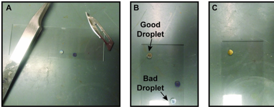
Figure 3. Process for making graphene liquid cells (A) Two graphene-coated TEM grids prepared on a glass slide with an edge cut off one of them. The surgical scalpel used to cut the grid is on the top right of the image. (B) Droplet of encapsulating solution on a graphene coated grid. The droplet on the top grid is the right size and has made a nice bead on the graphene. The droplet on the bottom grid has bled through the graphene, possibly due to a crack in the graphene. (C) Second graphene-coated grid placed on top of first grid with droplet of solution. This graphene liquid cell is now ready to load into a TEM. For size reference, the glass slide is 7.5 cm by 2.5 cm. Please click here to view a larger version of this figure.
