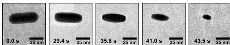
Figure 6. Gold nanorod etching in a graphene liquid cell pocket. Frames of a representative TEM video of a gold nanorod etching under dose rate of 800 \text{ e}^-/\text{Å}^2\text{s} . After an initial period of no etching, the nanorod etches at a constant rate. Please click here to view a larger version of this figure.
