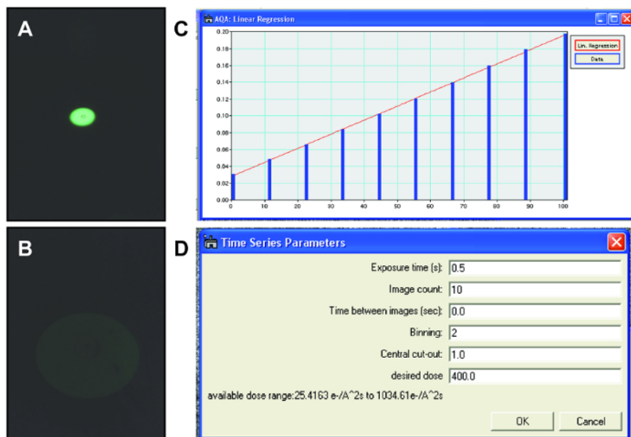
Figure 5. TEM beam control. (A) Condensed electron beam for dose rate calibration viewed using the fluorescent screen. (B) Expanded electron beam for dose rate calibration viewed using fluorescent screen. Intensity decreases as the electrons per area per time decrease which is why the electron beam is very faint. (C) Calibration curve relating the electron beam dose rate to the condenser lens current. This calibration curve is used for controlling the beam dose rate during imaging. (D) Parameters used when collecting TEM videos of nanoparticles in graphene liquid cells. Specific values used for each parameter may change depending on the material being imaged and the resolution needed. Please click here to view a larger version of this figure.
