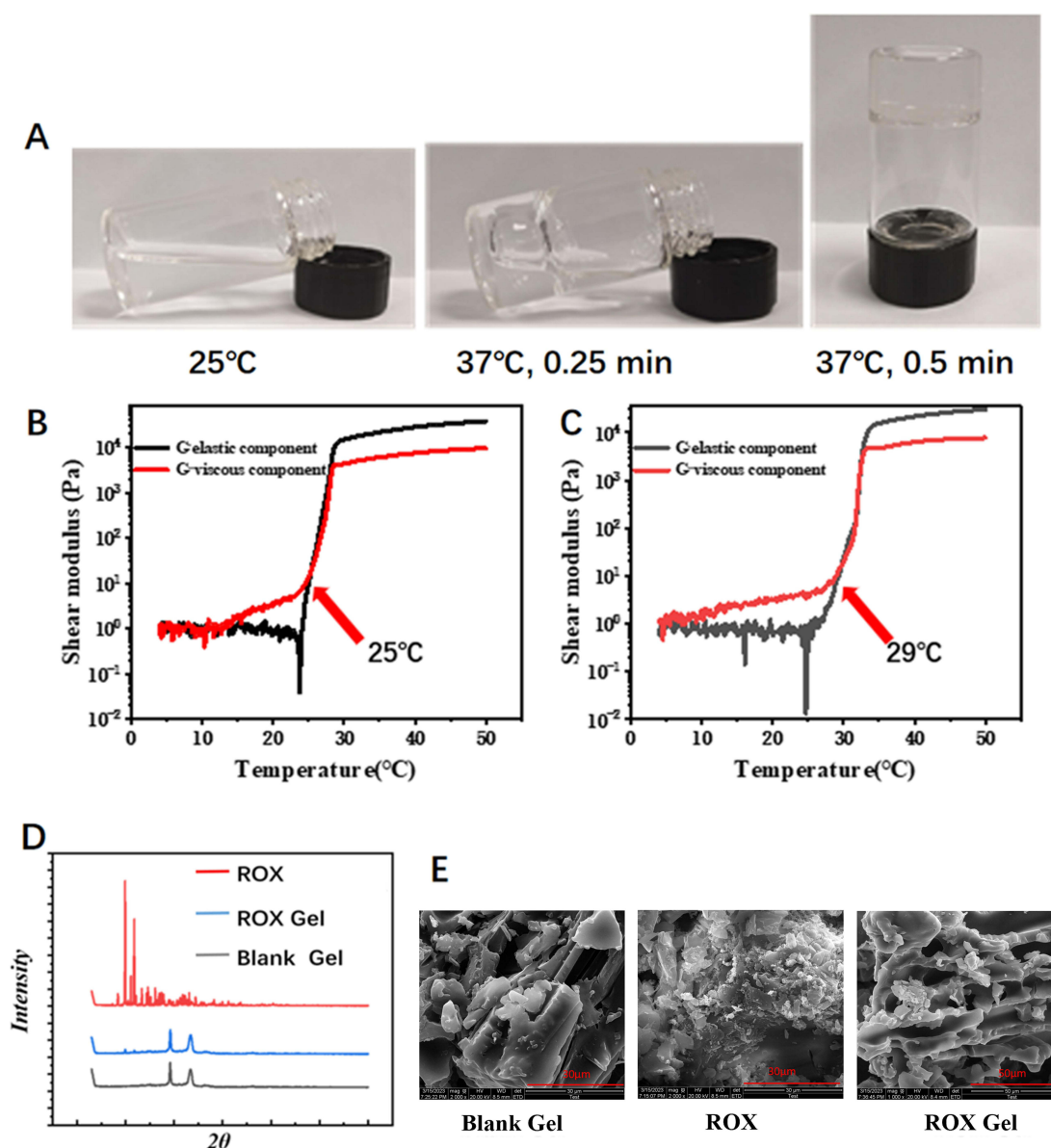
Figure 1 (A) Phase transition diagram of blank in-situ gel at room temperature and 37 °C. The changes of elastic modulus and viscous modulus with the variation of temperature for blank in-situ gel (B) and ROX in-situ gel (C). The XRD spectrum (D) and SEM images (E) for different samples. The scale bar is 30 μm.
