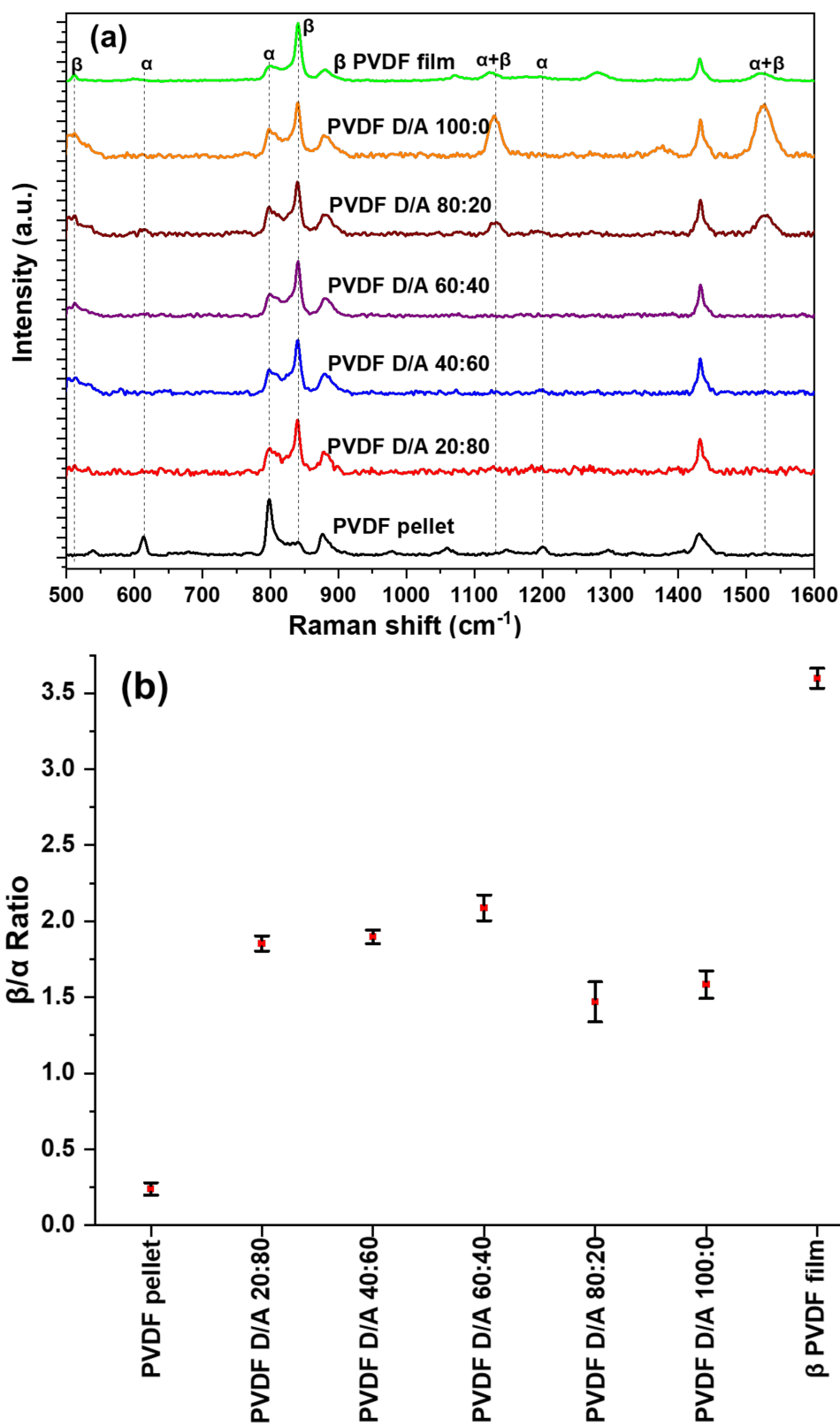
Figure 4. (a). Raman spectrums of electrospayed microparticles, PVDF pellet, and \beta -phase PVDF film (b) Average beta to alpha ratios of samples.
