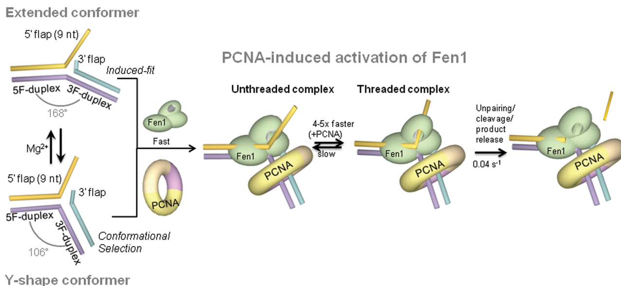
Figure 9. Model of PCNA activation of Fen1-substrate recognition. In the absence of protein, the substrate exhibits an Mg 2+ -dependent equilibrium between a Y-shaped structure and extended conformation with a [Mg 2+ ] 1/2 = 1.2 mM. Binding of Fen1 to the extended conformer induces a kink from 168° to 90–100° between the upstream and downstream duplexes (induced-fit model) and promotes opening of the flap junction. At moderate Mg 2+ ion concentrations (<2 mM), Fen1 could associate to the already bent Y-shape structure following a conformational selection model. After Fen1 binding to the flap base by establishing interactions with the downstream and upstream duplexes, the flap substrate threads through Fen1's helical arch. Association and dissociation rates are both slow but in the presence of PCNA, the association rate becomes 4-fold faster, suggesting a role in facilitating the flap threading step.
